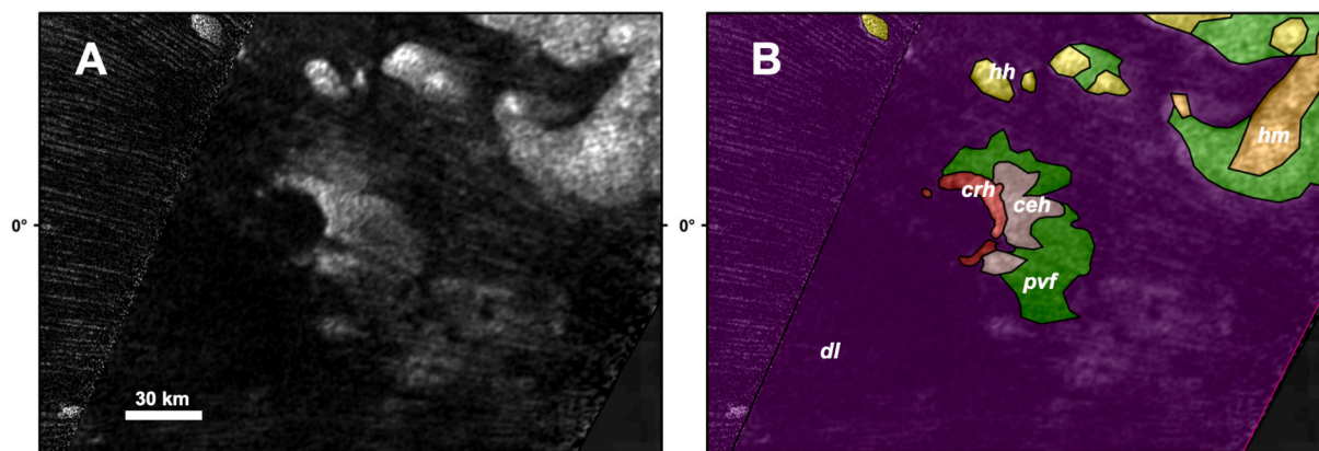
Fig. 14. Unnamed crater in South Belet (0.023°N, 79.51°W). (A) Unnamed crater in SAR. (B) Terrain unit mapping, including annotations of units.
