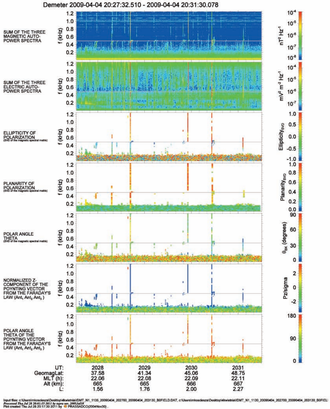
Figure 8. Detailed propagation analysis of a part of the ELF signal registered on April 4, 2009, as a function of time. Top to bottom: the two first panels show the spectrum of the magnetic and electric field variations (sum of the 3 components), the third panel shows the ellipticity of the magnetic field polarization. A value of 1 means right-hand circularly polarized waves; linear polarization gives 0; and -1 indicates left-hand circular polarization. The fourth panel is the sense of the polarisation of the waves, and the fifth panel indicates the angle between the Poynting vector and the Earth magnetic field, as calculated by the singular value decomposition technique [Santolík et al. 2003]. The bottom panel shows the z-component of the Poynting vector. Empty areas in the four bottom panels correspond to magnetic power-spectral densities below 10^{-7} \text{ nT}^2 \text{ Hz}^{-1} . In each panel, the black line is related to the proton gyrofrequency. The geomagnetic latitude and the magnetic local time (MLT) are displayed at the bottom of the figure according to the Universal Time (UT).
