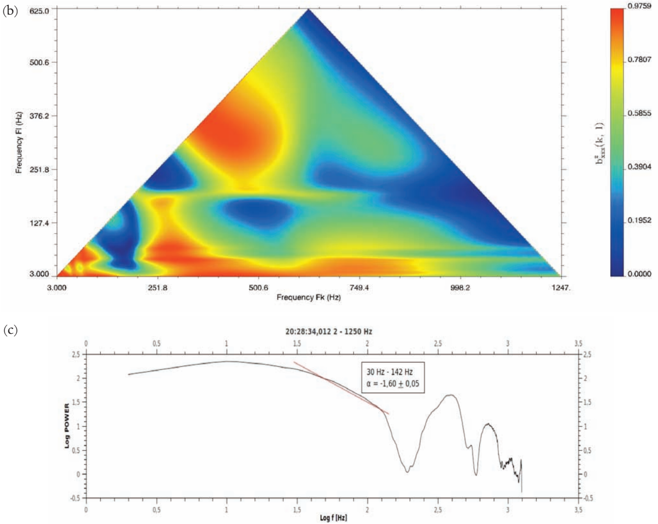
Figure 7b,c. (b) Bispectrum of the Ex signal in the ELF range. For description, see Figure 2b. The pattern of the frequency regions with strong 3-wave interactions is more complicated than for April 1. A clear picture of the turbulent cascade is seen in the lower part of the panel. (c) Single spectrum with slope \alpha \approx -1.60 .
