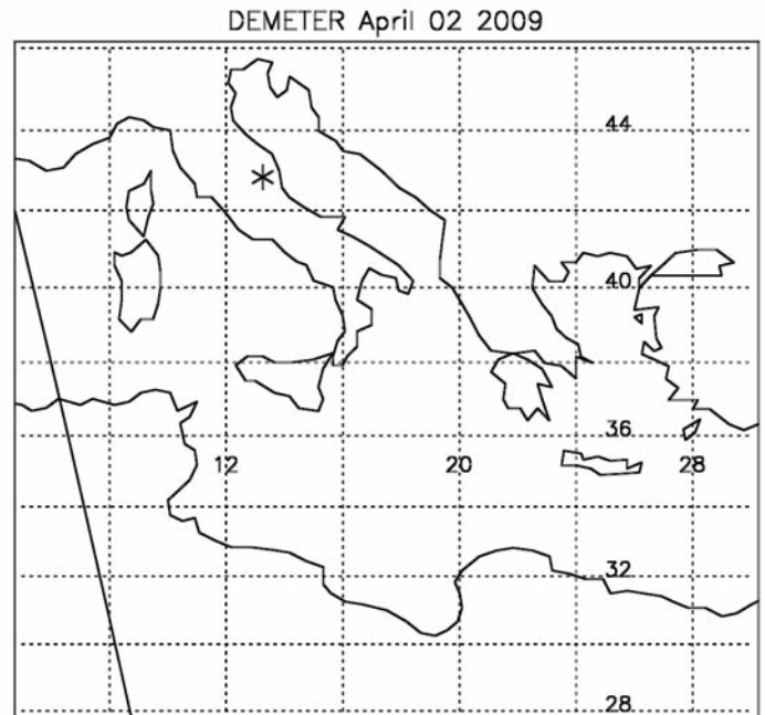
Figure 4. Map showing the epicenter of the April 6 L'Aquila earthquake (*) and the orbit of the DEMETER satellite on April 2, 2009. The point of closest approach from the epicenter was 60 km.
