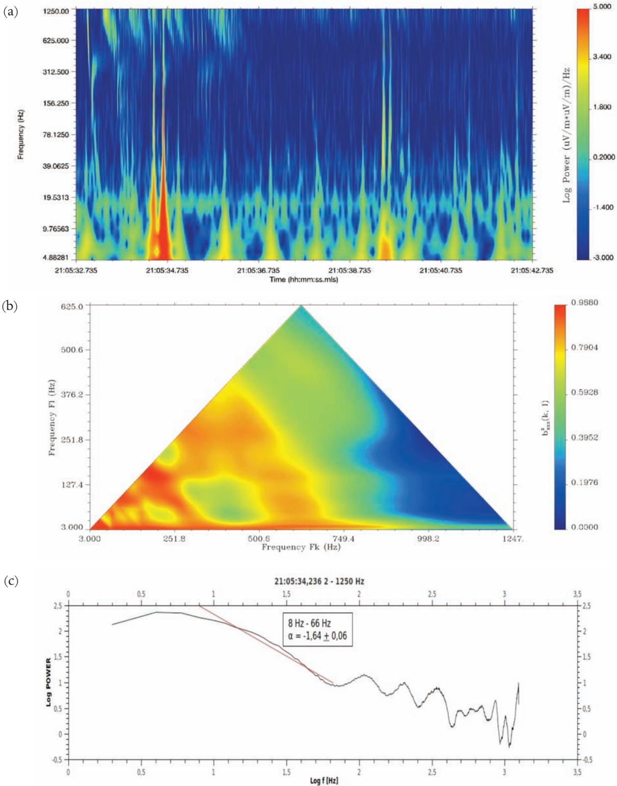
Figure 5. (a) Wavelet spectrogram of the broad-band emission in the ELF range at a greater distance from the epicenter (677 km), although still in the zone of seismic influence, in terms of a Dobrovolsky definition. The color scale is as in Figure 2. (b) Bispectrum of the Ex signal in ELF range. For description, see Figure 2b. The pattern of the frequency regions with strong 3-wave interactions is more complicated than for April 1, although a clear signature of the turbulent cascade is seen in the lower part of the panel. (c) Single spectrum with slope \alpha \approx -1.64 .
