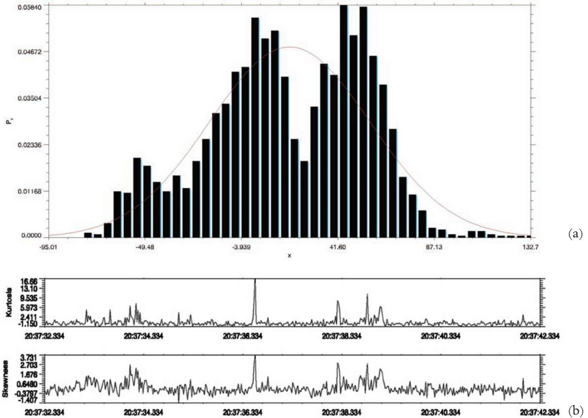
Figure 3. (a) Probability distribution function of the electric field intensity variations for the same time interval as in Figure 2. (b) Evolution of the kurtosis and skewness of the PDF between 20:37:32 and 20:37:42 UT.
