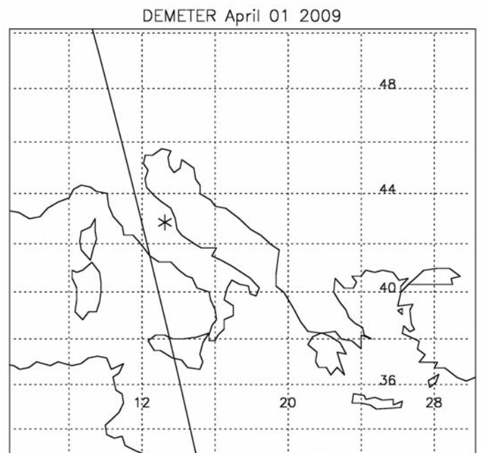
Figure 1. Map showing the epicenter of the April 6 L'Aquila earthquake (*) and the orbit of the DEMETER satellite on April 1, 2009. The point of closest approach is a larger distance from the epicenter (677 km).
