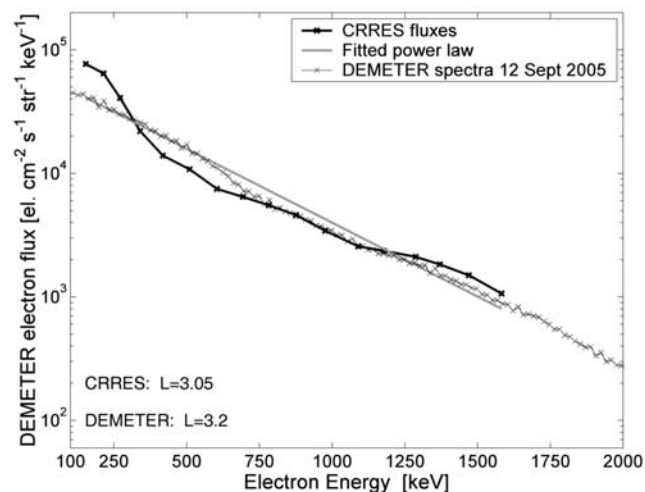
Figure 3. Electron energy spectra at L \approx 3 , typical of those seen following significant enhanced magnetic activity leading to enhanced trapped electron fluxes. The heavy line shows the trapped flux measurements by CRRES, with the gray line indicating a power law fitting. The thin line shows the contrast with the DEMETER-observed spectra in the drift loss cone, shifted to overlay with the CRRES fluxes.
