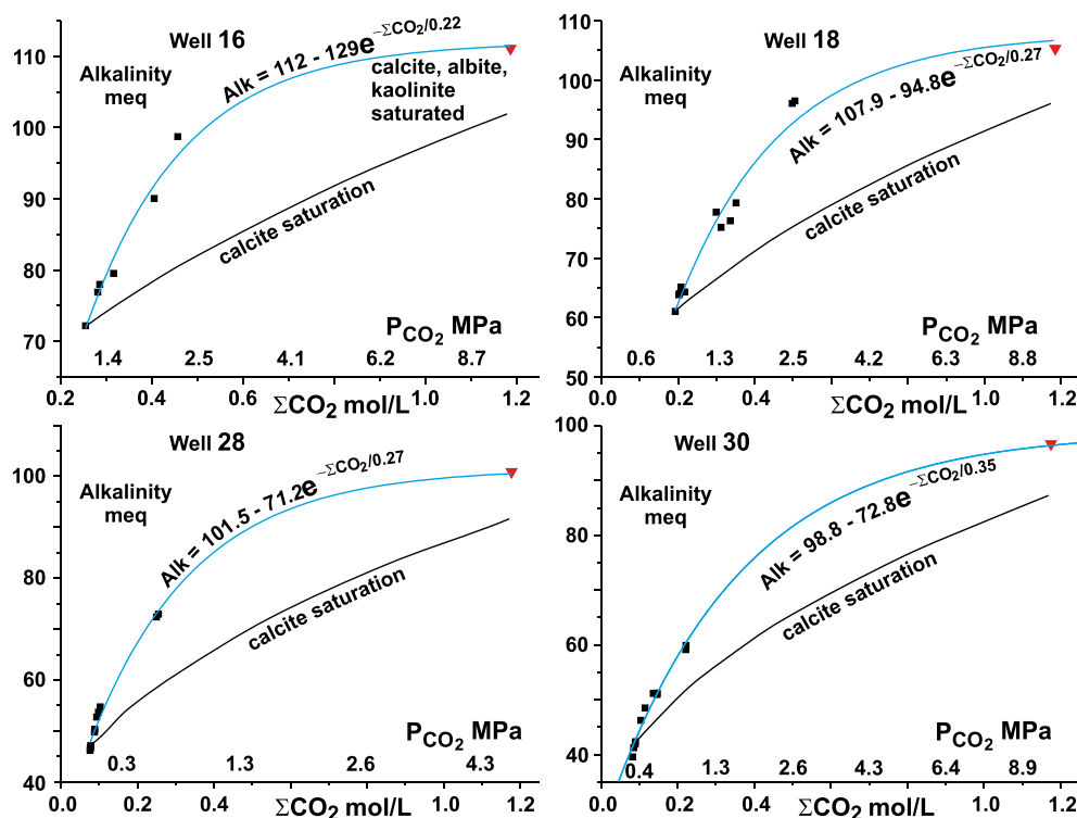
Fig. 17. Variation of alkalinity with total dissolved \text{CO}_2 ( \Sigma\text{CO}_2 ) for fluids from wells (points give average of groups of 5 samples) where total \text{CO}_2 is calculated from assumption that fluids are in equilibrium with calcite at reservoir pressure of 10 MPa and temperature of 50 °C. Lines labelled 'calcite saturation' show evolution of initial fluid (average of first five samples) as \text{CO}_2 partial pressure is increased while maintaining equilibrium with only calcite. Red triangle shows alkalinity of initial fluid brought to equilibrium with calcite, albite and kaolinite. Calculated using PHREEQC. Blue lines are best fit to well sample alkalinity data with calcite-albite-kaolinite saturated composition fixing high \Sigma\text{CO}_2 end of line. (For interpretation of the references to color in this figure legend, the reader is referred to the web version of this article.)
