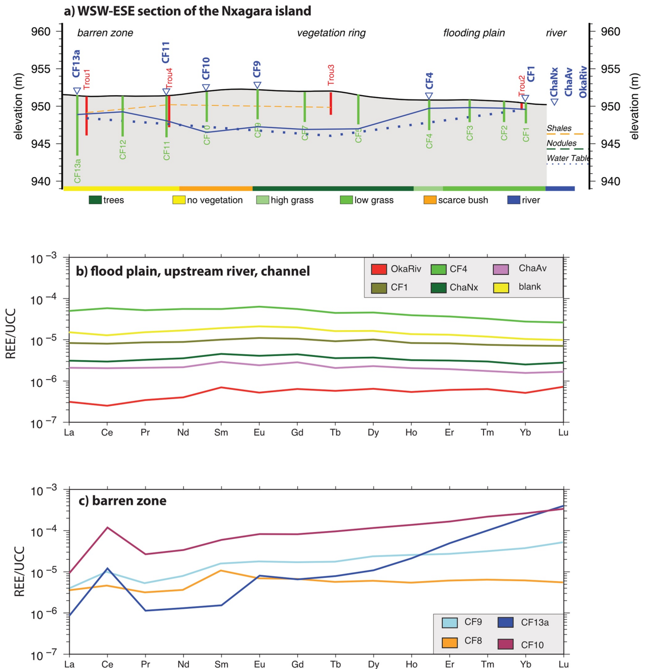
Figure 5. Rare Earth Elements patterns of the water sampled in the piezometers: (a) section of the Nxagara Island with the location of the piezometers and the vegetation distribution (the blue color shows the location of the water table, the orange line indicates the clay level and the dashed green line represents the nodule level), (b) in the floodplain, upstream in the river and channel, and (c) in the barren zone.
