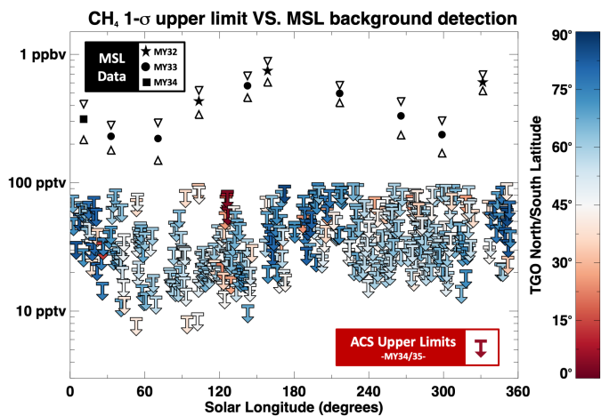
Fig. 8. Annual evolution of the best 1\text{-}\sigma upper limits (clipped at 100 pptv) derived at each occultation and plotted as a function of Solar longitude ( L_s ). Upper limit symbols (downward arrows) are coloured depending on their latitude. The values reported by MSL in Webster et al. (2018) concerning the background detections of methane are shown as filled stars (MY32), circles (MY33), and squares (MY34) with their associated error bars.
