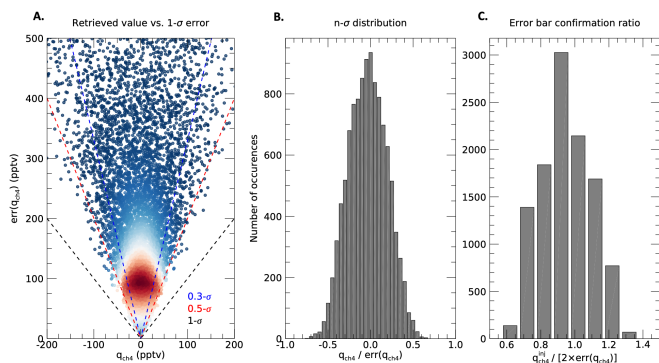
Fig. 4. (A) Retrieved CH 4 VMR values plotted against their corresponding 1- \sigma uncertainty, with colours referring to the density of points (redder equals denser), and the horizon corresponding to 0.3, 0.5, and 1- \sigma represented by the blue, red, and black dashed lines. (B) n- \sigma distribution of the retrievals, with n- representing the ratio of the retrieved value over its corresponding 1- \sigma error. (C) Distribution of the upper limit verification index, which is equal to the ratio of the CH 4 LOS density value retrieved after injecting an amount equivalent to the CH 4 2- \sigma error into the spectrum.
