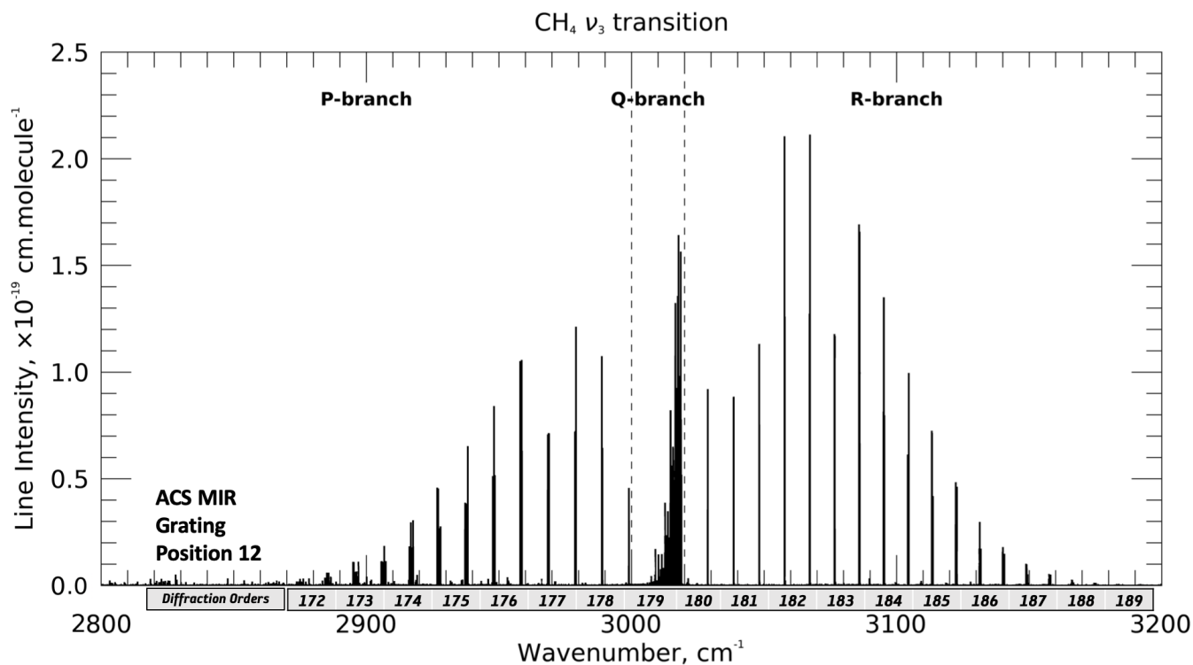
Fig. 1. The wavelength range used for the present study where the \nu_3 asymmetric C-H stretching vibration band of \text{CH}_4 is located. ACS spectral coverage is shown for indication with a discretization into spectral segments corresponding to the diffraction orders sampled by the grating position 12 set-up. The Q -branch, which comprises the densest portion of the band, is located in orders 179 and 180 whereas the most intense lines of the \nu_3 transition can be found in the R -branch and are sampled by order 182.
