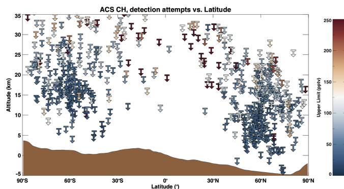
Fig. 7. Altitude distribution of 1- \sigma upper limits derived by ACS as a function of latitudes. Upper limit symbols are coloured depending on their value. Mars topography or zonal mean elevation with respect to MOLA zero datum is indicated with the brown shaded area.
