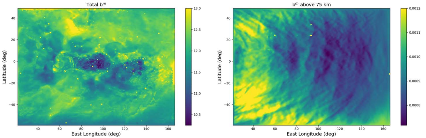
Figure 3. Left: the total gas optical thickness b^m of the Venus atmosphere. Right: the gas optical thickness of the atmosphere above 75 km. These optical thicknesses pertain to \lambda = 600 nm, and have been calculated for an afternoon pressure map of the Aphrodite Terra region (Lefèvre et al. 2020), as shown in Figure 1.
