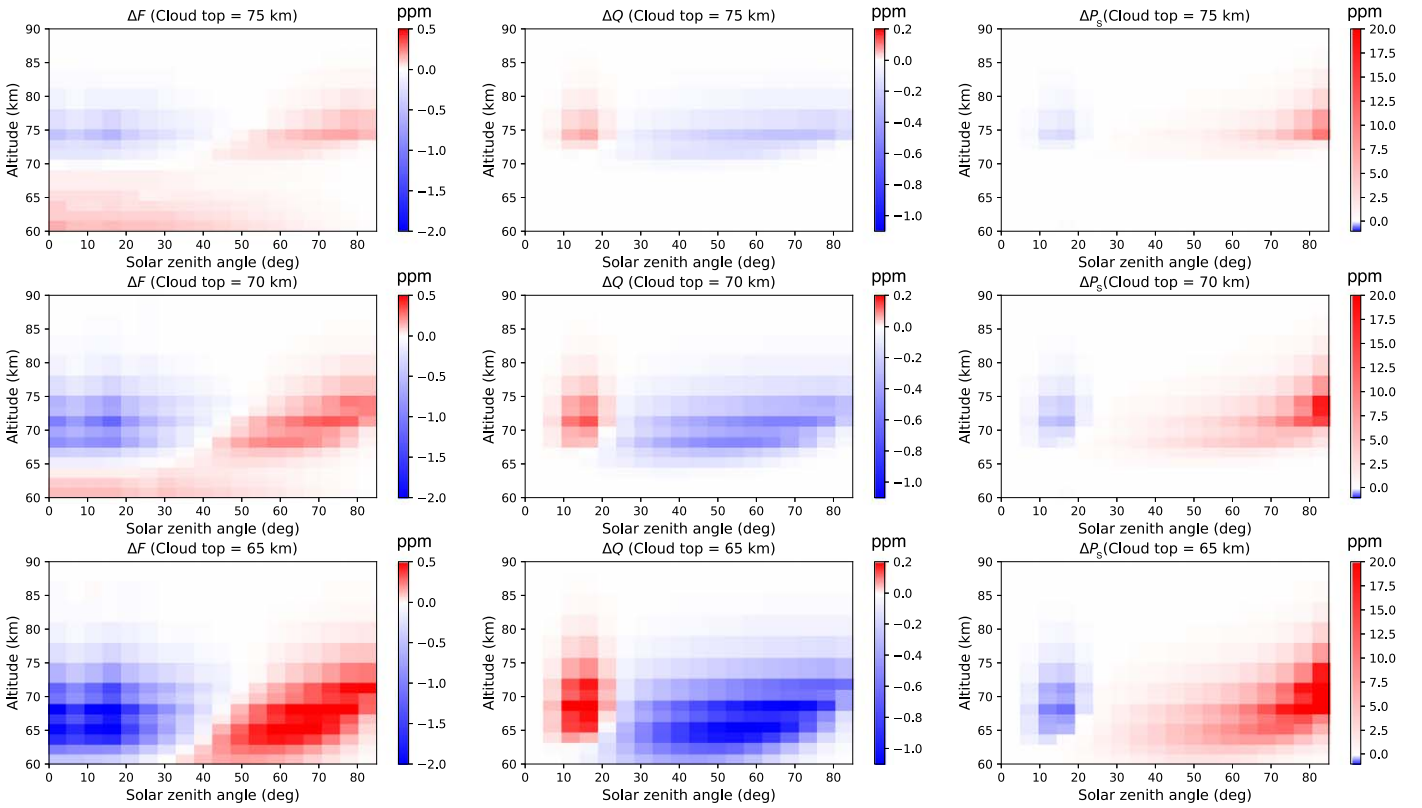
Figure 7. \Delta F (left column), \Delta Q (middle column), and \Delta P_S (right column; all in ppm) upon increasing the gas density or b_{\text{gas}}^m in an atmospheric layer by 1% as functions of \theta_0 for different cloud top altitudes: 75 km (top row), 70 km (middle row), and 65 km (bottom row). The cloud and haze scale heights are 4 km. The wavelength is 600 nm, and the viewing angle \theta = 0^\circ . A positive/red (negative/blue) color indicates an increase (decrease) in F , Q , or P_S with an increase in b^m .
