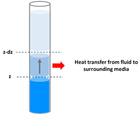
Figure 1: Diagram of the Control Volume used for heat transfer modeling inside the production borehole. Heat is either advected by fluid flow or conducted radially in the surrounding media.
