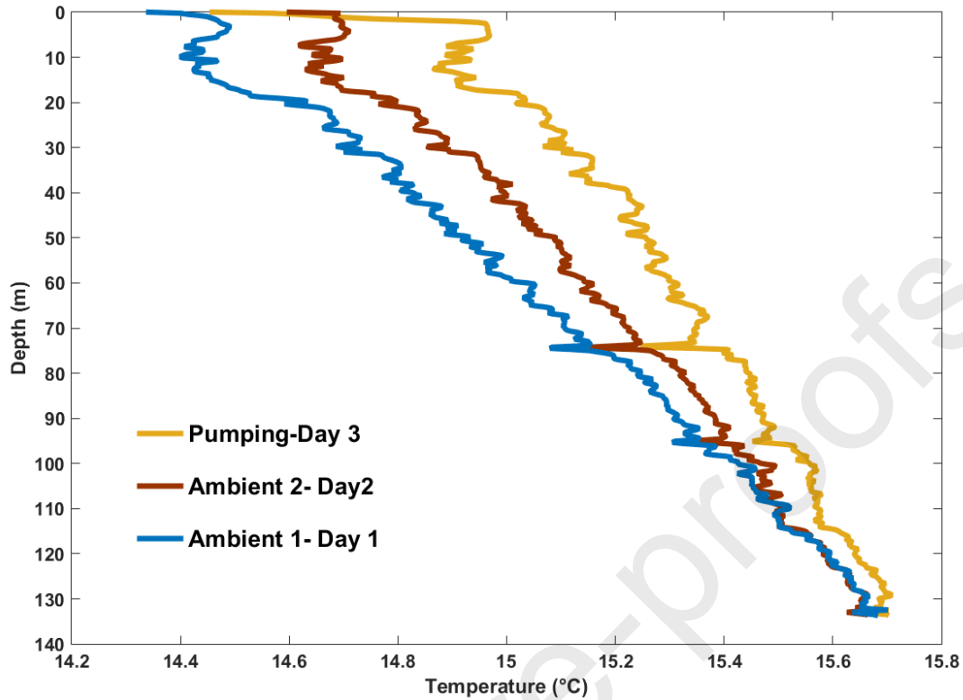
Figure 6: Comparison of three time-shots recorded temperature profile (smoothed) corresponding to the 3 different flowing conditions (ambient 1, ambient 2 and pumping).
