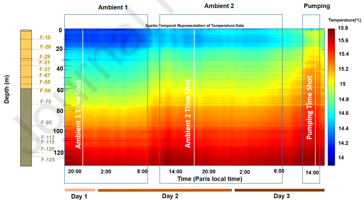
Figure 5: Representation of borehole schematic (left) with the position of the different fractures identified and Spatio-temporal temperature data (smoothed) recorded in borehole PZ-26 during the three different hydraulic conditions. The
