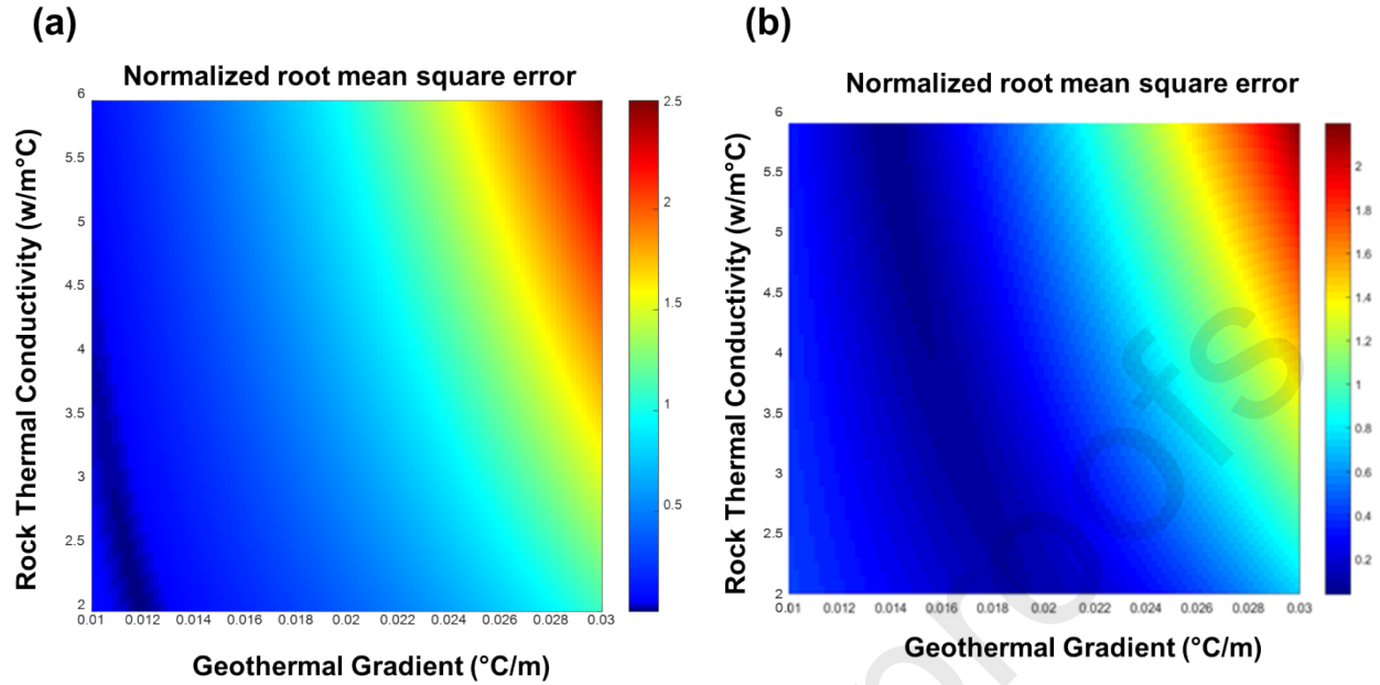
Figure 8: Normalized RMSE error between predicted flow by DTS and measured flow rate at the surface at (a) one-day flow time (b) six-months flow time
