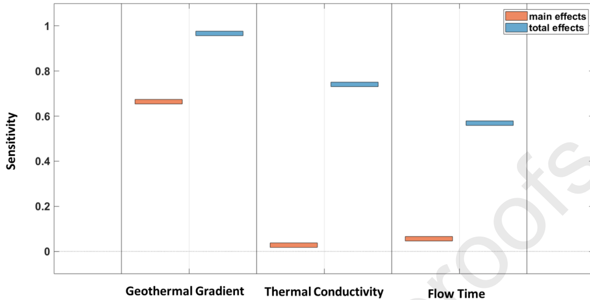
Figure 4: Global sensitivity analysis (Sobol method) performed for three parameters and the corresponding sobol indices including main effect and total effect. The main effect represents the contribution of parameter alone while the total effect represents its interaction with other parameters.
