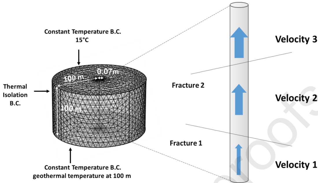
Figure 2: Schematic of the numerical model and representation of the borehole with two fractures and three flowing sections
