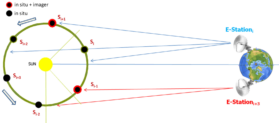
Fig. 5. Illustration of Earth-spacecraft communication and instrument activity. The deep space network at Earth consists of six antennas of which two ( E\text{-Station}_i and E\text{-Station}_{i+3} ) are operating simultaneously as displayed in the figure. Each Earth station is intermittently in contact with only three spacecraft, all spacecraft perform in-situ measurements whereas only two spacecraft also perform remote measurements (i.e. in-situ + imager), depending on their location.
