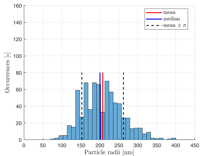
(b) 1%CH 4 tholins.
