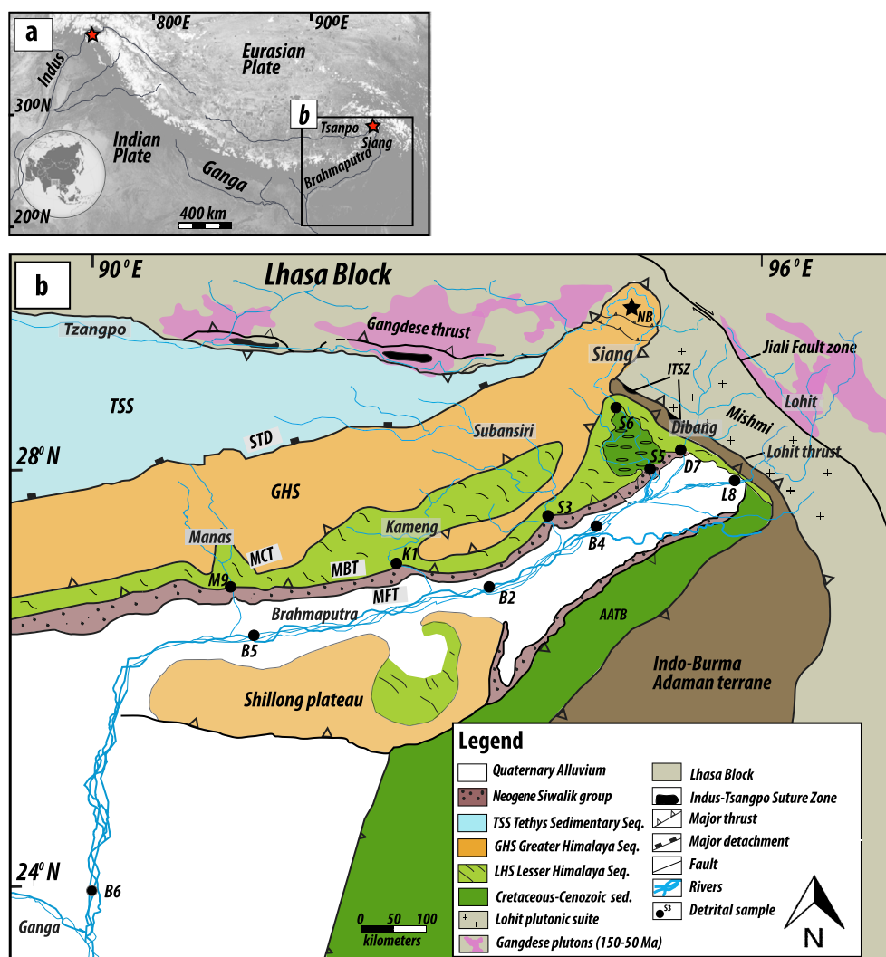
Fig. 1. Studied area in the eastern Himalaya. (a) Overview map, showing the major Himalayan rivers; western and eastern syntaxes are indicated by red stars. (b) Regional geological map (modified from Yin et al., 2010) showing the sample locations, the main tectonic features and the main rivers. Abbreviations: STD – South Tibetan Detachment; MCT – Main Central Thrust; MBT – Main Boundary Thrust; MFT – Main Frontal Thrust; ITSZ – Indus-Tsangpo Suture Zone; TSS – Tethyan Sedimentary Sequence; GHS – Greater Himalaya Sequence; AATB – Assam Akaram Thrust Belt; NB – Namche Barwa. (For interpretation of the colors in the figure(s), the reader is referred to the web version of this article.)
