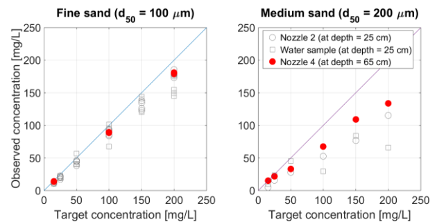
Figure 2. DEXMES provides homogeneous suspension for mud and fine sand (left). Vertical gradient in concentration and deposition occur for medium sand (right).
