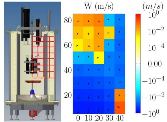
Figure 1. DEXMES device with 8 by 5 grid of ADV measurement positions and the velocity field obtained from ADV. Impeller speed is 175 rpm .
