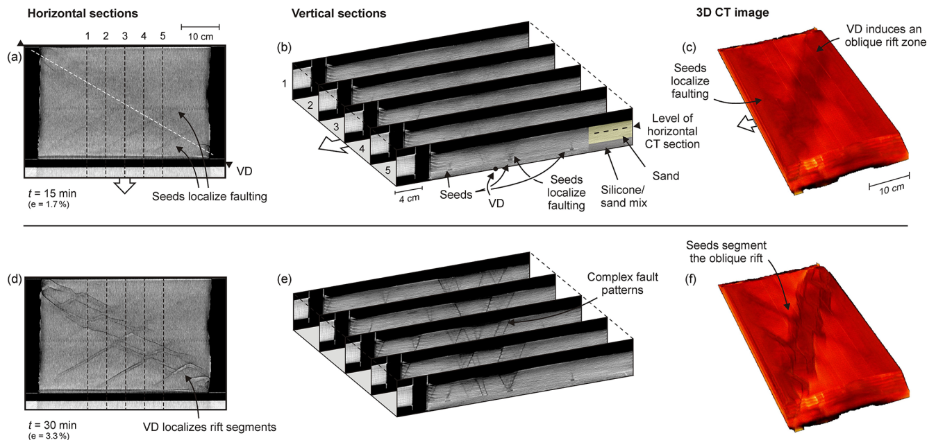
Figure 8. CT analysis of Model L (30° oblique VD, -30° oblique seeds, CT-scanned rerun of Model K). (a, d) Horizontal sections through the brittle layer. (b, e) Serial cross sections. (c, f) 3D CT images. Note that the colours in these images represent CT-scanning intensities and are not to be interpreted as a measure of model surface altitude.
