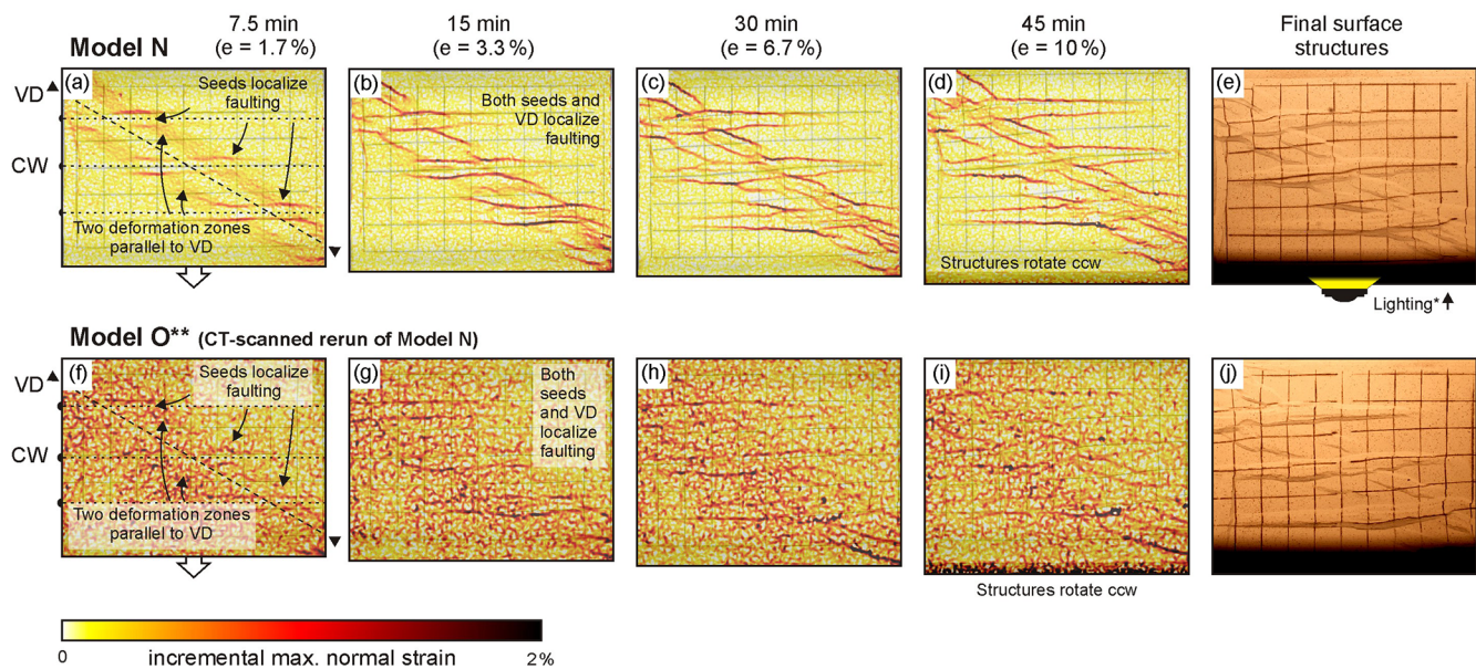
Figure 9. Incremental maximum normal strain maps of models N and O from Sub-series 2.3 (with 30° oblique VD, model axis-parallel weaknesses in the brittle cover and a double extension velocity of 40 mm/h; compare to reference models G and H, Fig. 5a–j) obtained through PIV analysis, taken as a proxy of fault activity. The increments for PIV analysis were 1 min, i.e. every 0.33 mm of extension. The original models map-view pictures are visible in the background. The right-hand column depicts the model surface at the end of each experiment. VD: velocity discontinuity. CW: (simulated) crustal weakness. ccw: counter-clockwise. * Shadows cast by one-sided lighting allowing a better visualization of the final surface structures. ** Due to technical issues, the PIV analysis of Model O is less detailed.
