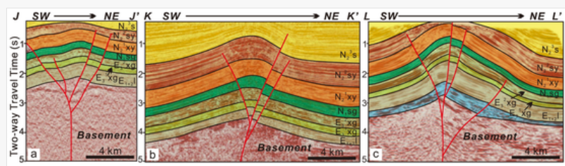
Reinterpreted seismic profiles in the western Qaidam basin. Location of each profile is shown in Fig. 9a. Original profiles are listed in Liu et al. (2019). Note the flower structures, indicating the strike-slip components along these basement-involved faults. E 1+2 1 xg; E 3 1 xg; E 3 2 xg; N 1 sg, N 2 1 xy, N 2 2 sy, N 2 3 s, Q 1 q are the abbreviated symbols for the Lulehe Fm., Lower Xiaganchaigou Fm., Upper Xiaganchaigou Fm., Shangganchaigou Fm., Xiayoushashan Fm., Shangyoushashan Fm., Shizigou Fm., Qigequan Fm., respectively.
