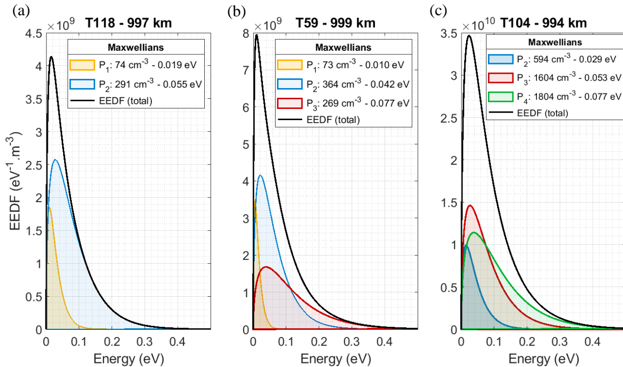
272 Figure 6. EEDF obtained from Maxwellian populations, at ~1000 km altitude for the flybys: (a) T118 273 (group G1); (b) T59 (G2); (c) T104 (G3).
