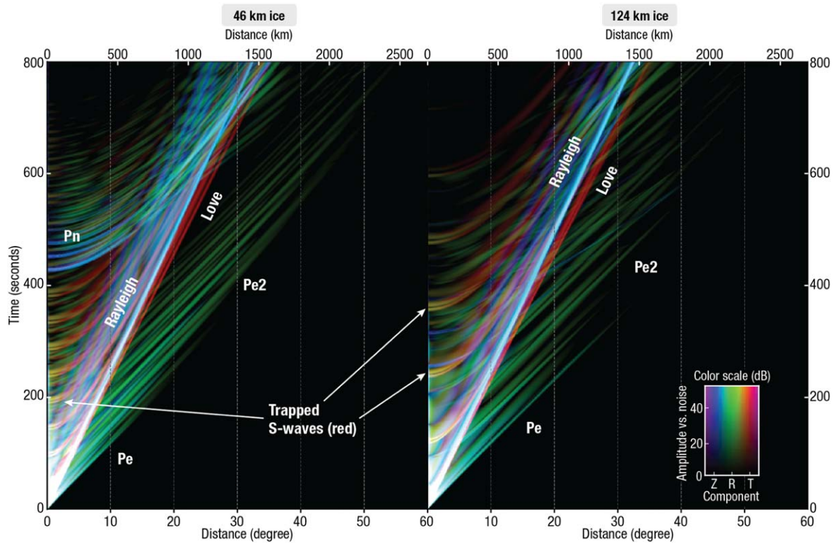
Figure 3. Simulated stacked seismograms for two Titan interior models: 46 km thick ice crust (left) and 124 km thick ice crust (right) over 410 km thick water ocean with 3.3% \text{NH}_3 (Panning et al. 2018; Stähler et al. 2018). Colors show the vertical (Z) and horizontal (radial and tangential) components of ground motion. The arrival times of Rayleigh and Love waves are a measure of source distance, while trapped S-waves indicate crustal thickness. The vertical gray lines at \sim 20^\circ indicate the approximate distance corresponding to the records shown in Figure 4.
