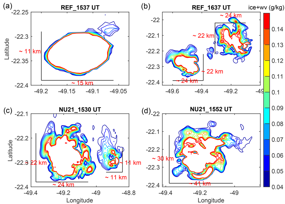
Figure 6. Size of the overshooting plumes at the 380 K isentropic level, shown for REF (a, b) at 15:37 UT and 16:37 UT, and NU21 (c, d) at 15:30 and 15:52 UT, respectively. These times are selected from Table 1. The colour contours show certain levels from 0.04 to 0.14 \text{g kg}^{-1} of total \text{H}_2\text{O} content to highlight the outer part of the overshooting plumes. The solid black lines give the approximate range of each figure in kilometres.
