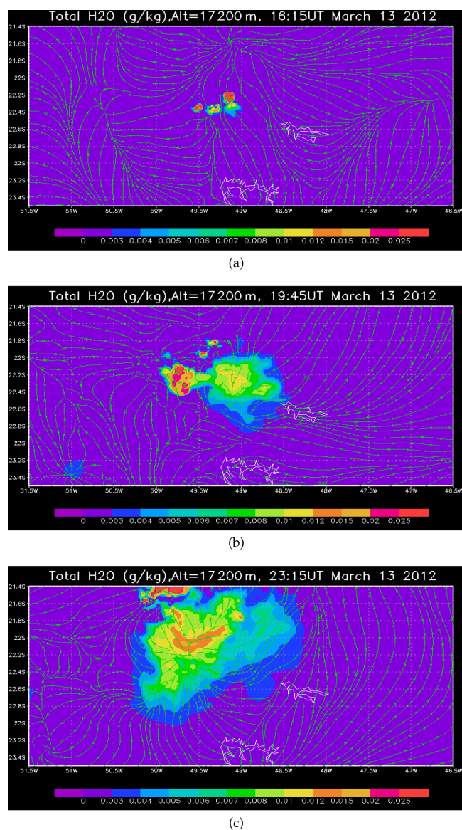
Figure 2. BRAMS simulation: REF total water content, ice, liquid, and vapour in \text{g kg}^{-1} , at 17.2 km altitude at (a) 16:15 UT, (b) 19:45 UT, and (c) 23:15 UT, respectively. The streamlines represent the horizontal wind fields within the domain, a composite of the second and third grids.
