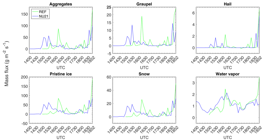
Figure 7. The instantaneous domain-average mass-flux rate ( \text{g m}^{-2} \text{s}^{-1} ) of each hydrometeor and water vapour is illustrated in the third grid of the simulations for REF (green) and NU21 (blue). The cosine component of the vertical velocity with respect to the horizontal is used to determine the upward flux rate, which takes into account the slope at the 380 K level due to deep convection.
