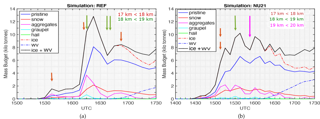
Figure 8. Water mass budget (ice and water vapour) for (a) REF and for (b) NU21 in the third grid between the 380 and 430 K isentropic levels. The ice budget contribution includes the five ice hydrometeors (pristine ice, snow, aggregates, graupel, and hail). The colour and length of the arrows indicate the cloud-top altitude of each occurrence, with the smallest arrows (brown) referring to cloud-top heights of 17–18 km, the intermediate-sized arrows (green) relating to cloud-top heights of 18–19 km, and the largest arrows (magenta) corresponding to cloud-top heights greater than 19 km.
