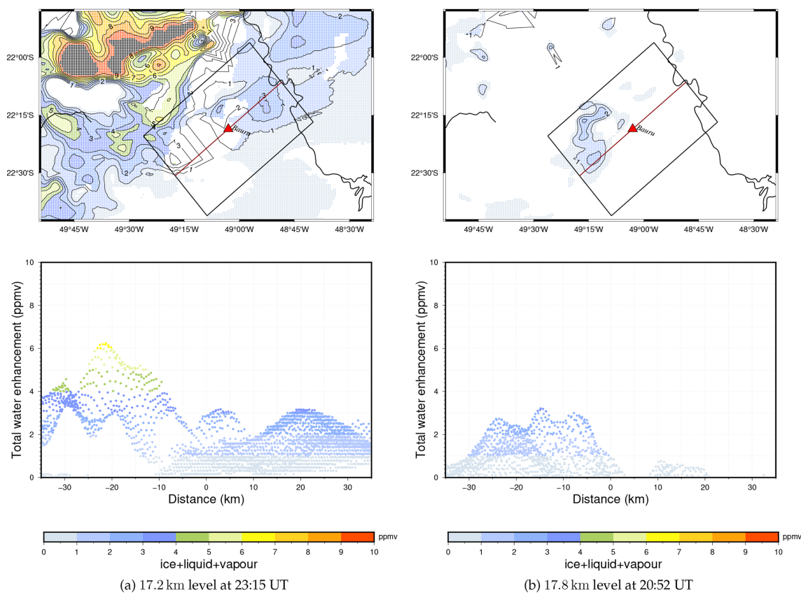
Figure 3. REF providing total water (ice, liquid, and vapour) enhancement at (a) 17.2 km altitude at 23:15 UT and (b) 17.8 km altitude at 20:52 UT, respectively. The top panel shows the horizontal cross sections of the vertical grid at these altitudes, depicting the only grid points when their total water content is higher than the model levels simply above and below in a vertical column. The isolines show the enhanced total water content (ppmv) with respect to the model layer below it. The bottom panel shows the grid points'/pixels' water content confined by the northeast-tilting rectangle having the length of 70 km and half width of 25 km. The red triangle denotes Bauru (0 km); the northeast direction is positive, and vice versa.
