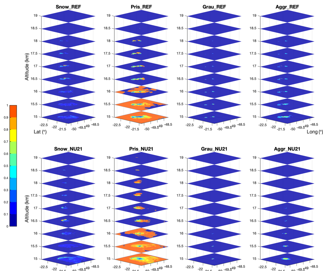
Figure 5. Vertical distribution of horizontal cross section of hydrometeors, viz., snow, pristine ice, graupel, and aggregates, within the third grid, spanning over 15–19 km altitude. It is for the ratio of four types of ice hydrometeors against the entire ice content from REF – upper panel, and NU21 – lower panel, shown at 16:15 UT. Hail is not included because of its negligible values within the plume.
