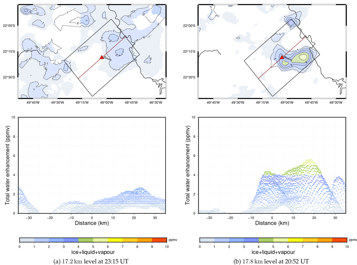
Figure 4. Like Fig. 3 but representing NU21.
