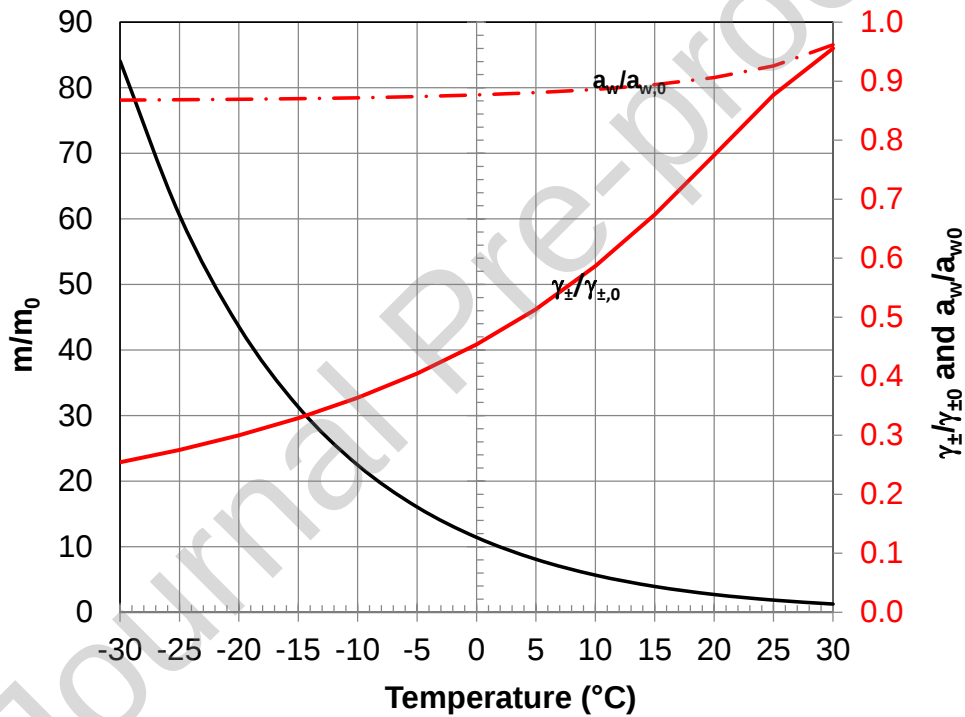
Figure 9. Ratio from thenardite values over mirabilite's, on the sulfate ion molality ( m / m_0 ), mean activity coefficient ( \gamma_{\pm} / \gamma_{\pm,0} ), and water activity ( a_w / a_{w,0} ), calculated with Pitzer correction according to the ColdChem database [24].
