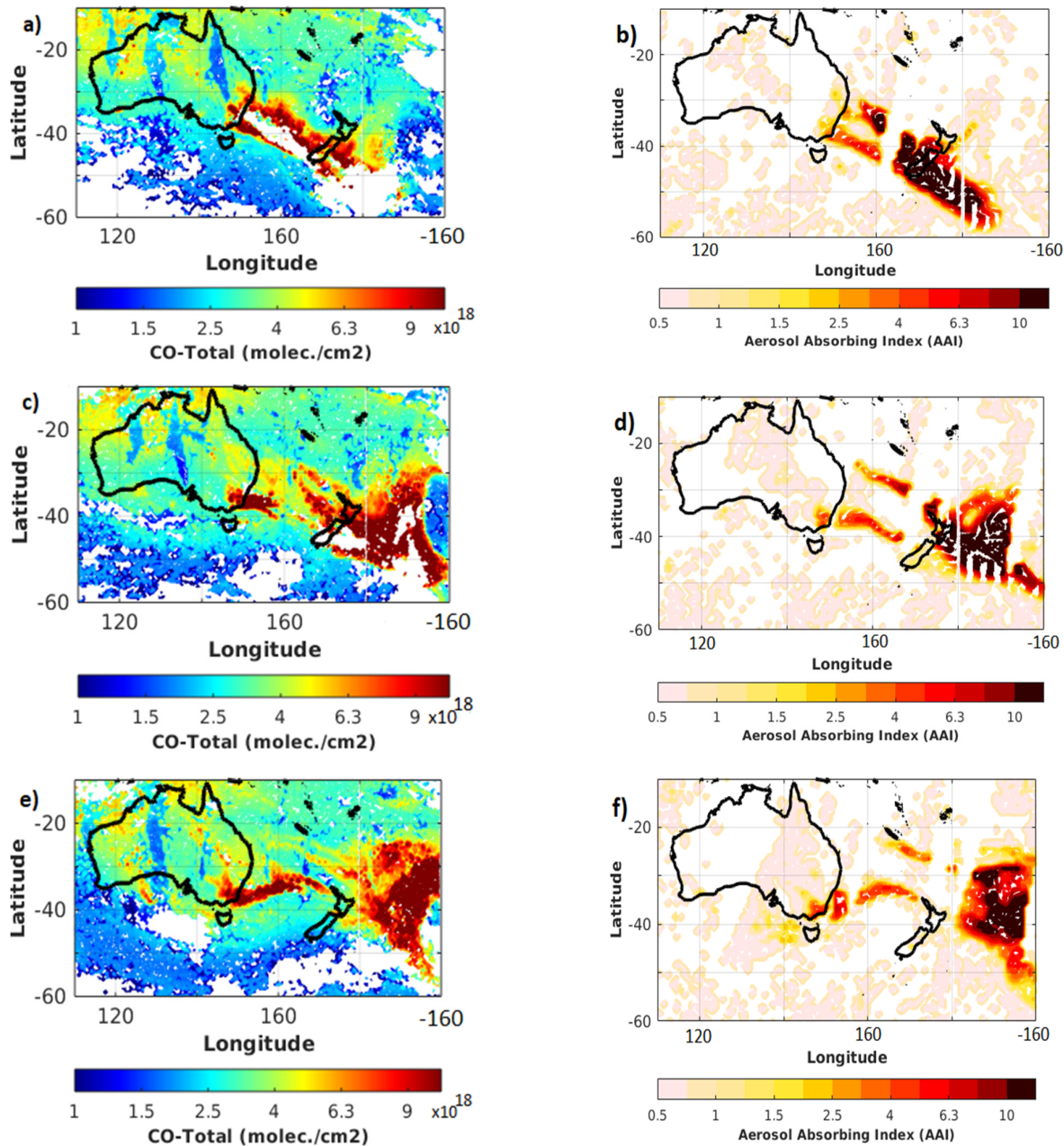
Figure 4. Daily maps of CO total columns (a,c,e) obtained from IASI observations and AAI (b,d,f) from GOME-2 observations recorded on the 31 December 2019 (top), 1 January 2020 (middle) and 2 January 2020 (bottom).
