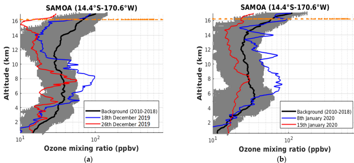
Figure 9. OMR profiles obtained from ozone radiosonde measurements performed at Samoa on (a) December 2019 and (b) January 2020. The monthly mean profile and the associated standard deviation calculated during the 2010–2018 period are in black lines and grey areas, respectively. The tropopause height is indicated by the orange horizontal lines.
