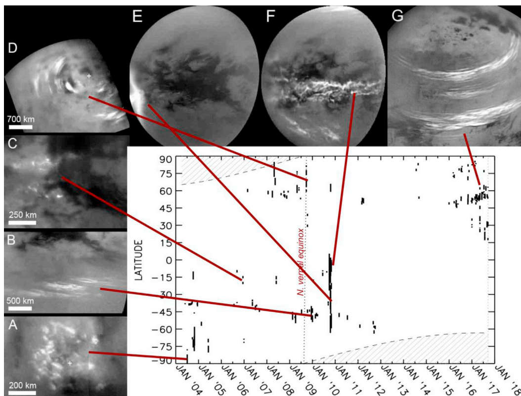
Fig. 9. Cassini ISS images of different types of clouds (A–G) and graph of the latitudes at which clouds have been observed over the mission, spanning May 2004–September 2017 (after Turtle et al., 2017).
