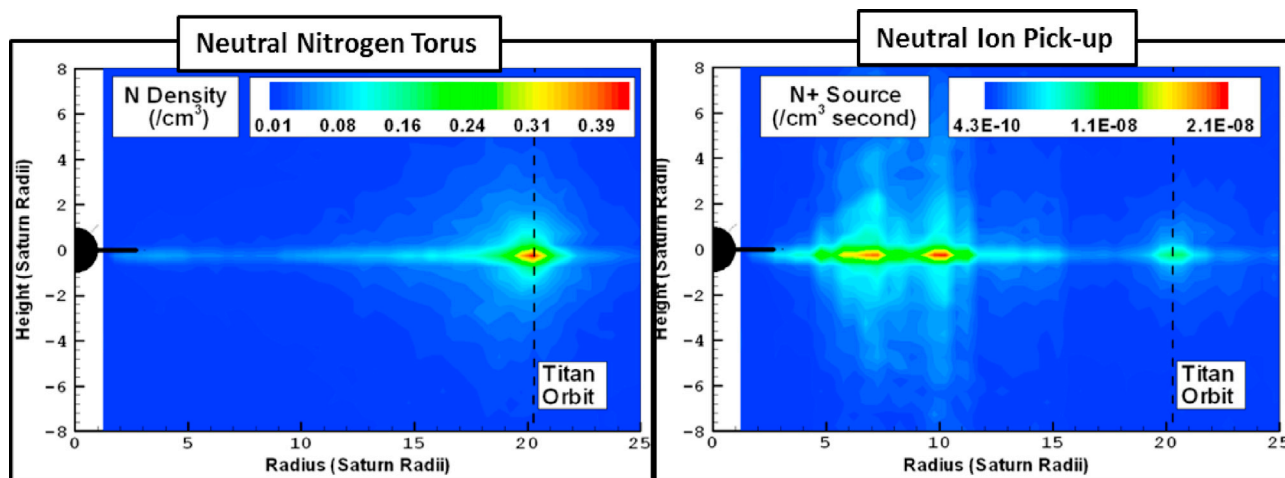
Fig. 13. Pre-Cassini nitrogen distribution models (derived from Smith et al., 2004). Left panel: Neutral N torus ( /\text{cm}^3 ) in R vs. Z coordinates ( R_s ). Right panel: \text{N}^+ pick-up ion source from the torus ( /\text{sec cm}^3 ) in R & Z coordinates ( R_s ). Although the peak neutral density is near the source, Titan, peak ion generation is in near the middle magnetosphere where electron densities and temperatures favor ionization. Due to the ambiguity in observations, it is possible this model could still be accurate or the torus may not exist at all.
