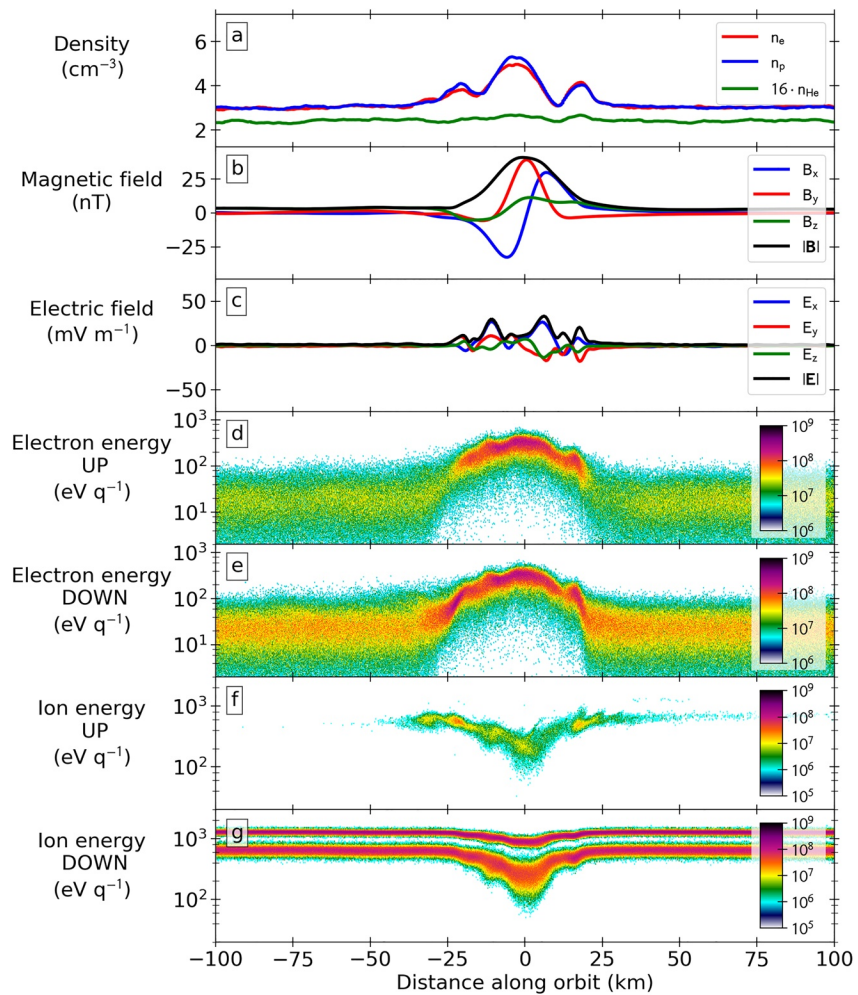
Figure 2. Line plots along the polar ( Y direction; magenta) orbit indicated on Figure 1. The differential energy flux (color scale in the lower four panels) has units \text{eV cm}^{-2} \text{s}^{-1} \text{sr}^{-1} \text{eV}^{-1} . All lines and distributions are snapshots recorded at the same time step after the simulations have reached steady state.
