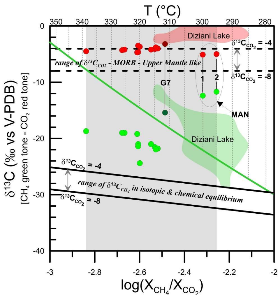
Figure 7. \delta^{13}\text{C} for \text{CO}_2 (red) and \text{CH}_4 (green) versus \log(X_{\text{CH}_4}/X_{\text{CO}_2}) of Mayotte bubbling gases. Dark red and green symbols are referred to the G7 sample of Milesi et al., (2020) mentioned in the text, also the red and green area are referred to the variability of the Diziani lake samples from the same authors. The green line correspond to the \text{CH}_4 and \text{CO}_2 thermal equilibrium expressed in equation (7) (Giggenbach, 1992), the thick black lines are calculated as the equation (9) for isotopic and chemical equilibrium between \text{CH}_4 and \text{CO}_2 for two cases of \delta^{13}\text{C}(\text{CO}_2) corresponding at -4\text{‰} and -8\text{‰} which in turn are indicated as dashed lines.
