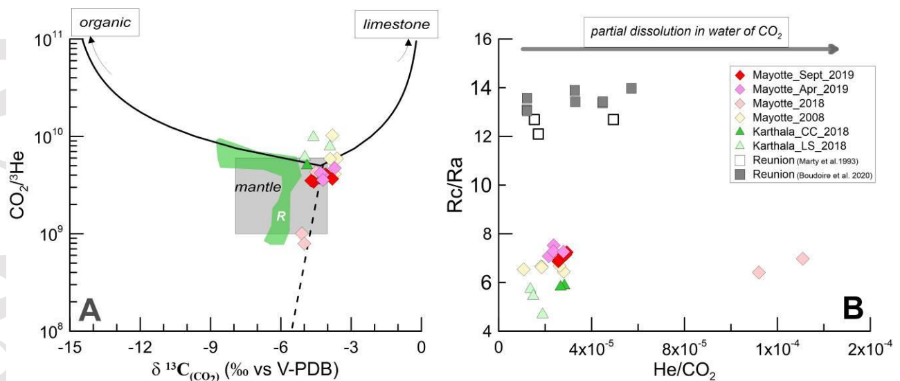
Figure 4. A: \delta^{13}\text{C} of \text{CO}_2 versus \text{CO}_2/{}^3\text{He} diagram of fumaroles and bubbling gases at Grande Comore and Mayotte. B: \text{He}/\text{CO}_2 versus \text{Rc/Ra} . For comparison is indicated also the variability of corresponding gases at La Réunion (R). Diagram 4A shows that gases at Comore archipelago are in the field of Mantle-like origin with no evident organic or limestone contributions. Solid lines are mixing curves between organic, mantle and limestone endmembers, while the dashed line indicates a Rayleigh fractionation dissolution. Diagram 4B displays a variable degree of water-gas interaction affecting \text{CO}_2 variability.
