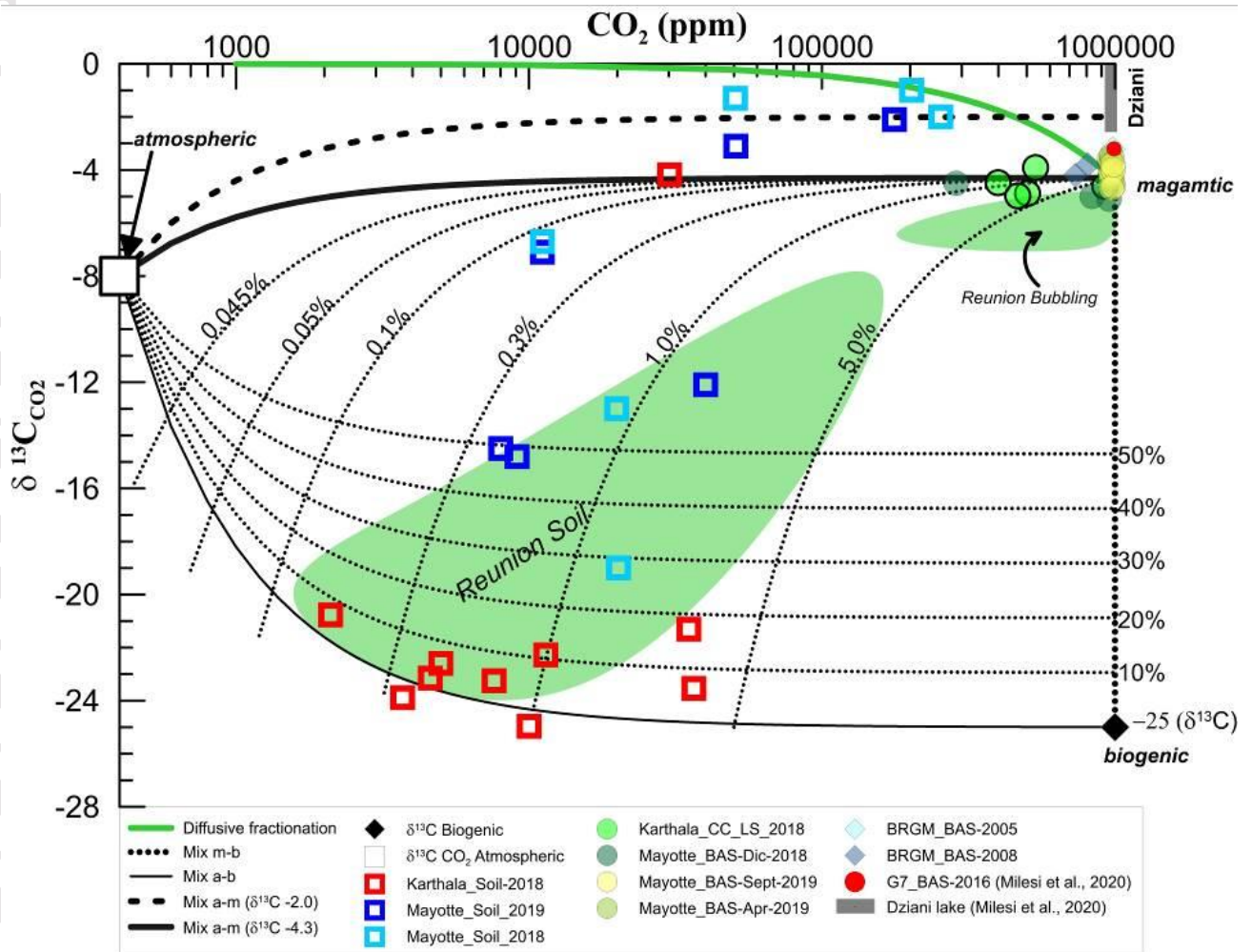
Figure 9. Diagram plotting carbon isotopic composition of soil \text{CO}_2 versus soil \text{CO}_2 log-concentrations (ppm) showing the theoretical binary mixing curves between three endmembers: atmospheric, biogenic and magmatic. Also shown are the binary mixing curves (hyphen curve) which allow a differentiation in the percentage of the magmatic component (M) in the hypothesis that the biogenic contribution could be extended up to \delta^{13}\text{C} 25‰ (Hoefs, 2015). Green areas are referred
