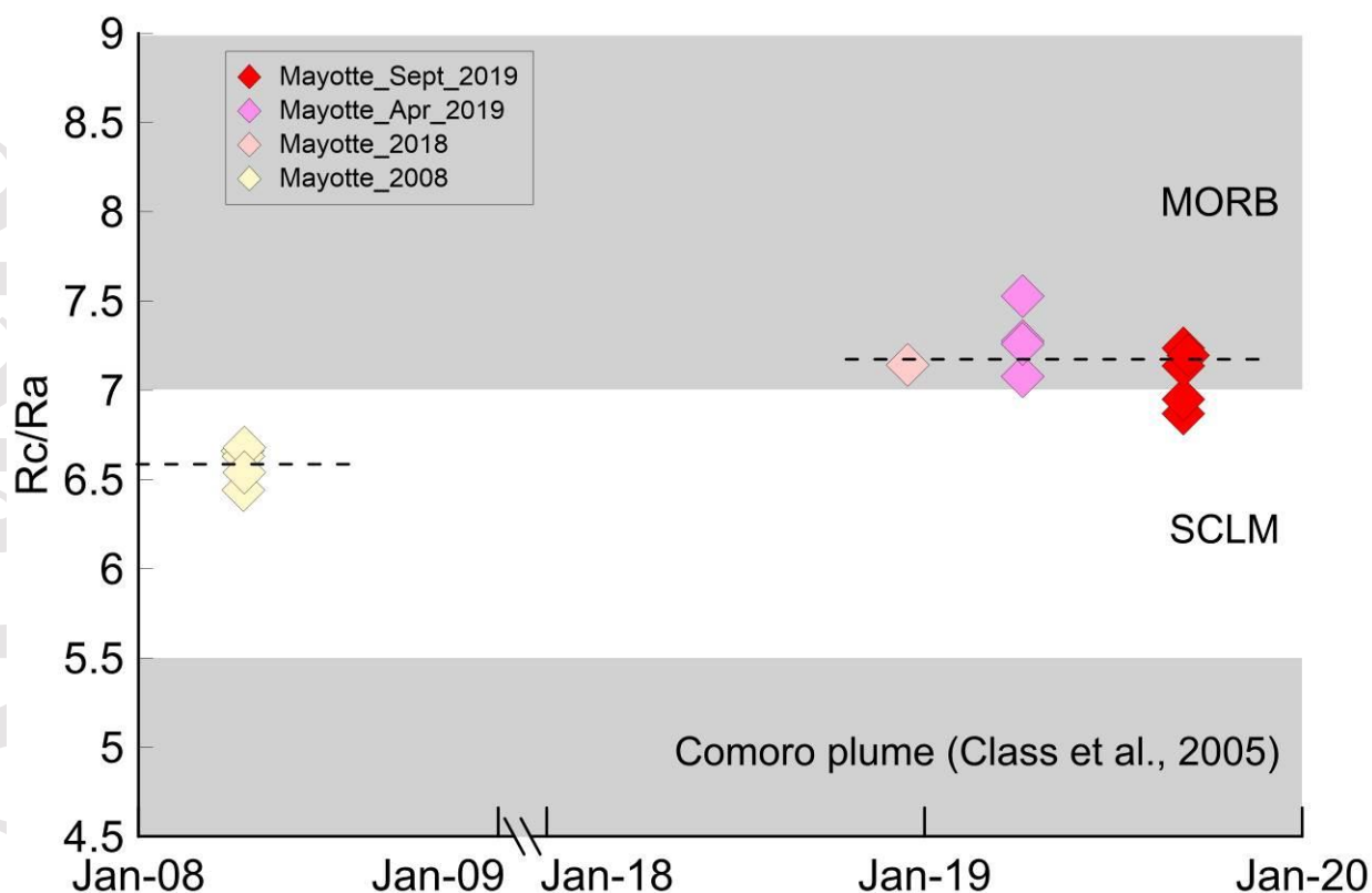
Figure 8. Rc/Ra time series. Rc/Ra has increased by an average 0.5 of between 2008 and 2018-2019. Black dashed lines indicate the averages Rc/Ra for the two distinct periods.
