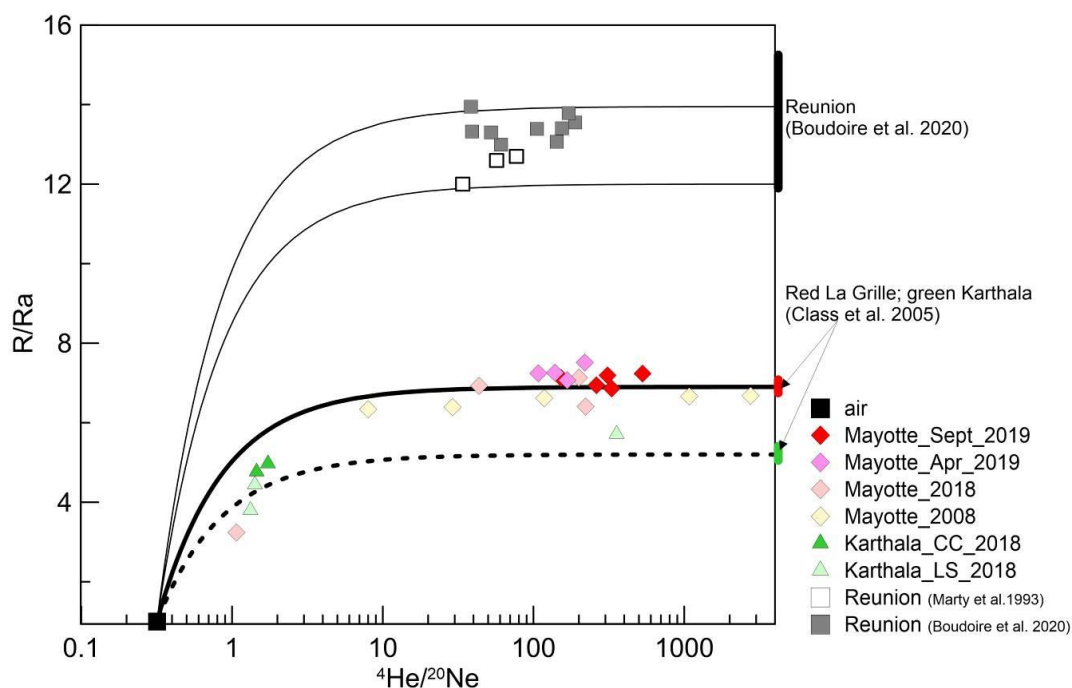
Figure 3. ^4\text{He}/^{20}\text{Ne} versus ^3\text{He}/^4\text{He} (R/Ra) in fumaroles and bubbling gas from Grande Comore and Mayotte. For comparison are shown data from bubbling gases at La Reunion from Boudoire et al., (2020) and Marty et al., (1993). Thick and dash black lines indicating air-magma mixing are calculated from the average value [from Class et al., (2005)] of La Grille and Karthala fluid inclusions respectively. Thin black lines are calculated as the minimum and maximum of bubbling gases at La Reunion. At the right side of the diagram are also indicated three solid black red and green bars, corresponding to the range of the R/Ra variability of La Reunion, La Grille and Karthala fluid inclusions respectively.
