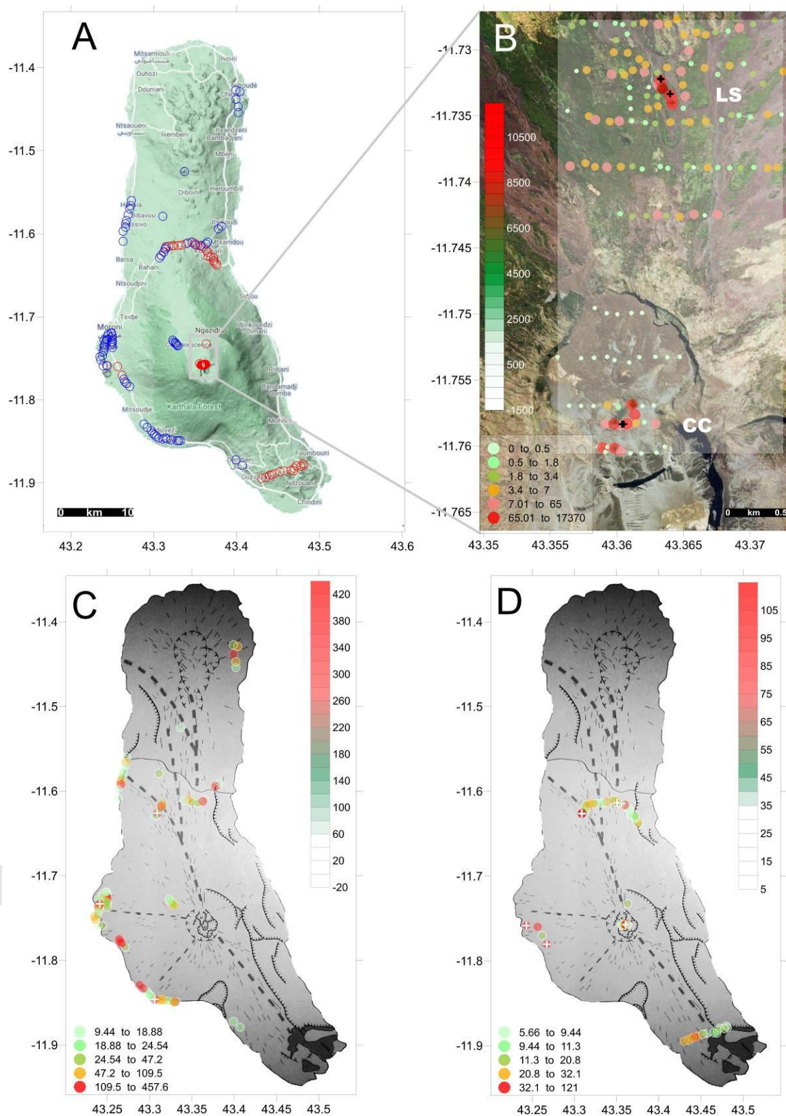
Figure 5. Soil CO 2 measurements at Grande Comore. In A sites of measurements distinct in blue and red for 2017 and 2018 surveys respectively (this study). Inside the white rectangle are indicated the 2018 sites of measurements not indicated in B. In figure 7B a classed post map (where soil CO 2 flux is expressed in range of g m -2 d -1 ) and a contour plot of soil CO 2 emission of the 2014 survey at the summit of Karthala volcano realized using the accumulation chamber method. CC indicates the Central Caldera area; LS indicates La Sufriere; the sites of the gas sampling of 2018 reported in table1 are indicated as black crosses. Figures 7C and D are related to 2017-2018 surveys respectively realized using the “Dynamic concentration method” [Gurrieri and Valenza (1988)]; the white crosses in 5B and 5C are the sites of soil
