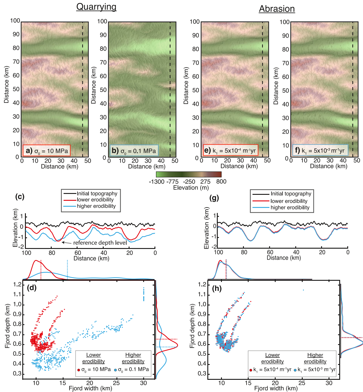
Figure 3. iSOSIA fjord models considering various bedrock erodibility with quarrying and abrasion laws. (a and b) Erodibility is set by varying \sigma_0 for quarrying (Equation 4) and (e and f) varying by an order of magnitude k_1 for abrasion (Equation 1). (c and g) Cross-sectional views of the resulting fjords shown along one transect downstream. (d and h) Fjord widths against depths for the respective models. The marginal distributions for width and depth are shown, with dashed lines corresponding to the mean of each distribution with similar colors. The parameter m (Equation 4) is kept constant ( m = 2.7 ).
