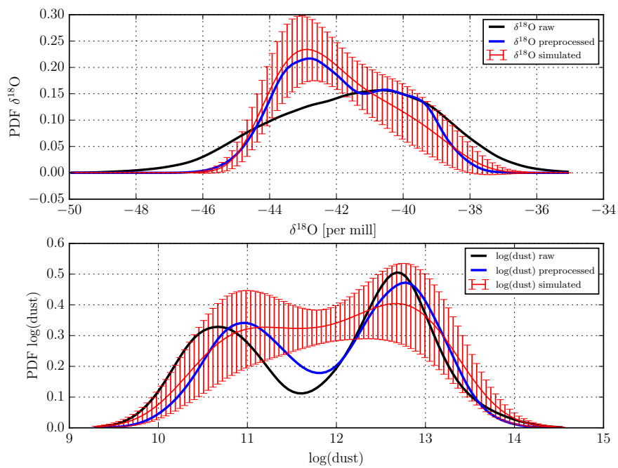
Figure A7. Same as Fig. 3a and b in the main text but for the model without coupling terms.
