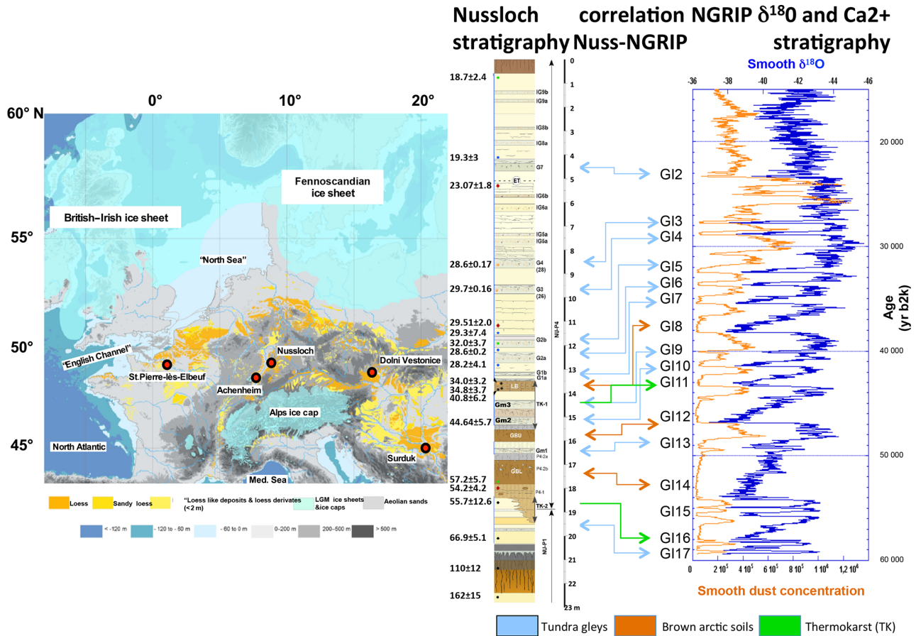
Figure 2. Stratigraphic correlations between Nussloch paleosols and NGRIP interstadials (GIs) (modified from Rousseau et al., 2017). Map as in Fig. 1. \delta^{18}O (‰, in blue) and the dust concentration (part/ \mu L, in brown) records in the NGRIP ice core over the interval between 60 ka and 15 ka b2k. Nussloch stratigraphic column from Antoine et al. (2016) modified.
