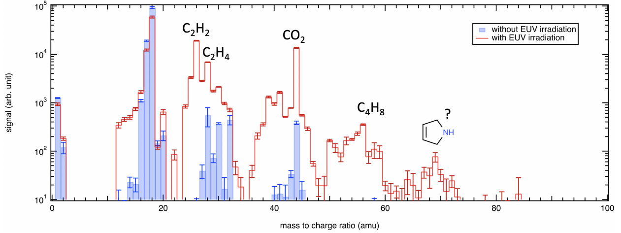
Fig. 2. Ex situ experimental m/z spectra obtained for neutral species with a N_2 - CH_4 - H_2O gas mixture with (red) and without (blue) irradiation in the photochemical chamber by using a 3-hour cryogenic trapping system.
