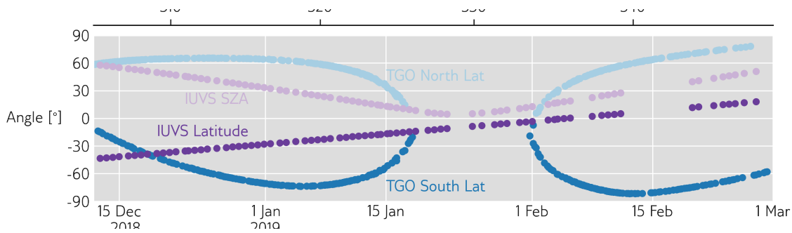
Figure 4: Geometry of TGO and IUVS observations shown in Figure 1. Points show the Mars surface geometry of the point along the observation line of sight with minimum ray height. For TGO, occultations are made in both hemispheres, but Figure 1 shows only Southern Hemisphere data. MCS observations are made at 3 PM across all latitudes, and zonally averaged across longitudes, and so are not shown here. Both TGO and IUVS observing geometry evolved with time over the period of the study, with minimal impact on the conclusion that regional storms can make possible large amounts of high-altitude water that subsequently increases coronal H abundances and loss rates.
