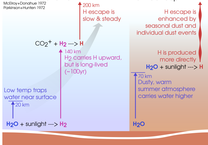
Figure 2: Paradigm for dust-driven and seasonal vs. impulsive escape at Mars. (left) In the traditional scheme, H loss is regulated by the slow-and-steady diffusion of molecular hydrogen to the upper atmosphere, with minimal changes in the loss rate with season or lower atmospheric conditions. In the emerging paradigm for H loss, seasonal or impulsive changes in dust can loft water to high altitude where it can directly boost escape. (top right) H loss from Mars peaks in Southern Summer because of seasonal changes associated with the solstice and perihelion, increased interhemispheric circulation, greater average dust activity, and greater insolation. (bottom right) For this work, we are able to distinguish impulsive loss due to the C-type dust event from seasonal loss because this event and its associated H loss enhancement occurred in the declining phase of the known seasonal trend. Determining the conditions under which impulsive H loss dominates seasonal or quiescent loss should be a focus of ongoing and future studies.
