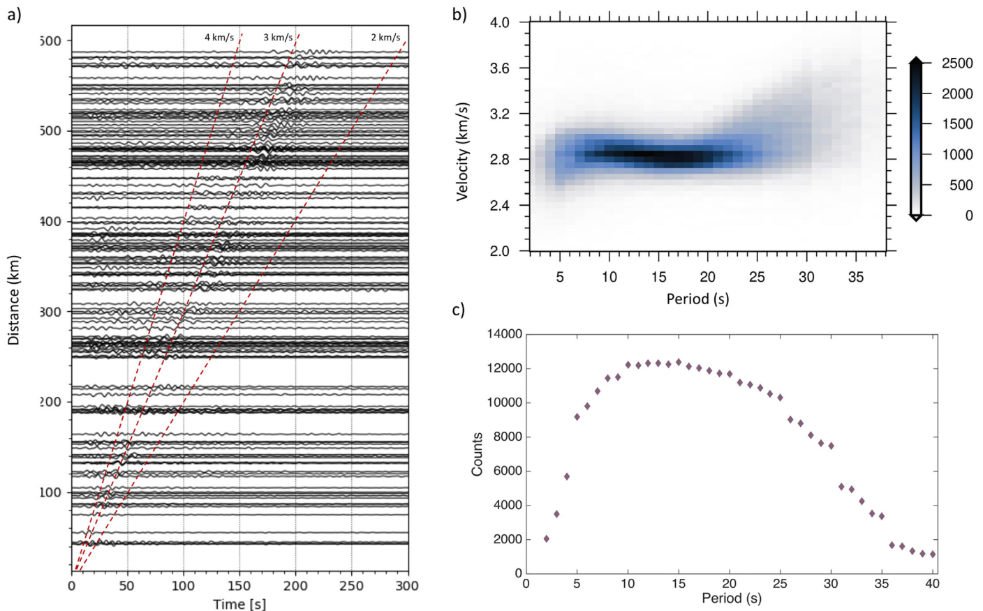
Fig. 2. (a) Example of cross correlations between CH.BERNI station and the other stations used in this study. The dashed lines denote velocities of 4, 3, and 2 km/s; (b) density plot of the group-velocity dispersion measurements as a function of period; (c) number of measurements for each period.
