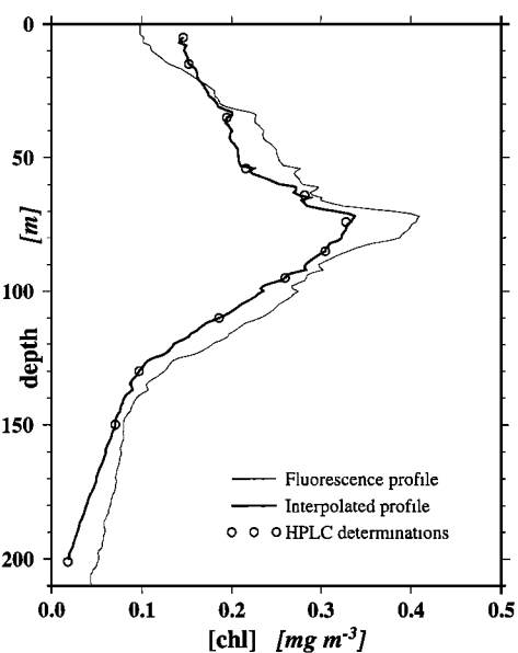
Figure 1. Example of the transformation of the in situ fluorescence profile into chlorophyll a (monovinyl and divinyl) profile based on HPLC discrete determinations made at 12 levels (OLIPAC, 150°W, 5°S, November 19, 1994).
