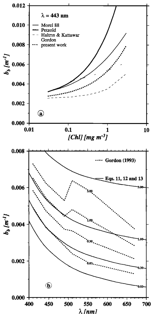
Figure 15. (a) Evolution of the backscattering coefficient at 443 nm with [Chl] , according to various parameterizations [Gordon et al. , 1988; Haltrin and Kattawar, 1991; JGR88] (see also Petzold's phase function used in conjunction with (9)). (b) Spectral b_b values for various [Chl] , according to Gordon [1993] (tabulated by Gregg et al. [1993]) and (11), (12), and (13).
