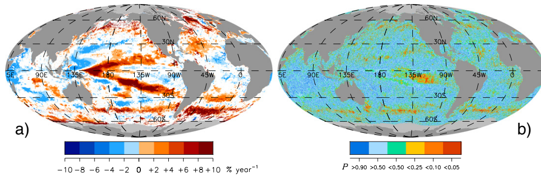
Fig. 8. a) Trends for OC-CCI Chla over the period Aug. 2002–Jul. 2011 (only significant trends, p < 0.05 , represented), and b) level of significance P of the t -test comparing the slopes of linear regression obtained for MERIS and OC-CCI over that period. Grey shows land, while light-grey is associated with areas where the series are insufficient for analysis.
