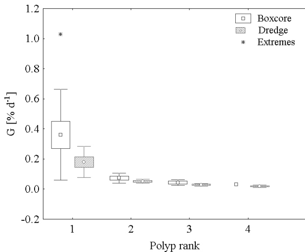
Fig. 2. Calcification rates ( G ) of Mingulay corals collected by box core or dredge as a function of polyp rank. Box and whiskers are \pm S.E. and \pm S.D., respectively.
