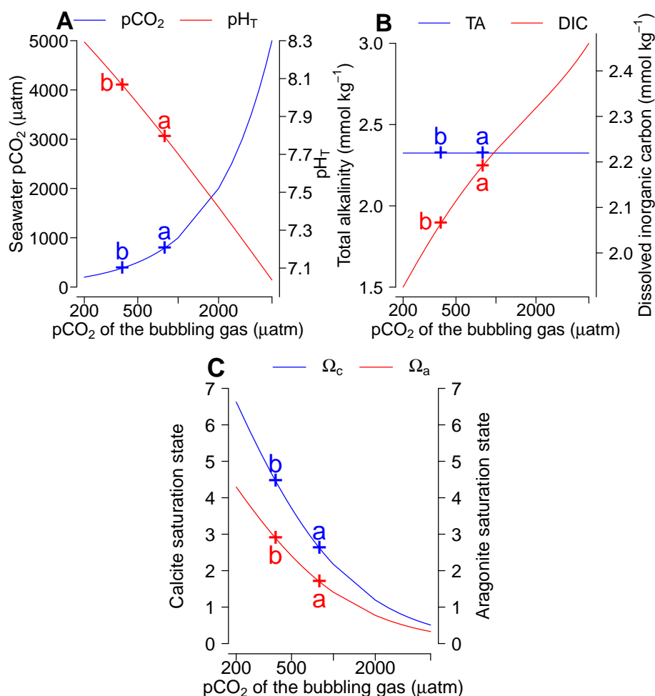
Fig. 1. Effect of bubbling seawater with gases of varying pCO 2 on the carbonate chemistry of seawater as computed with the seacarb function ppgas . The letters “b” and “a” indicate, respectively, the value of a parameter before and after perturbation for the example described in the text.
