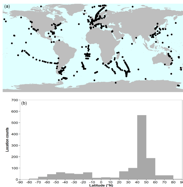
Figure 2. (a) Location of organisms and natural communities from which data has been archived and (b) distribution of locations according to latitude.
