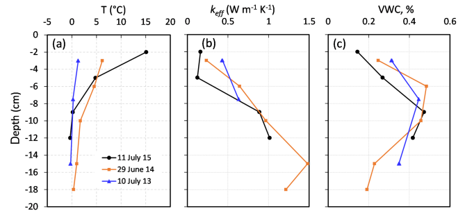
Figure 4. Vertical profiles of soil physical variables in pits dug in the polygon where our instrument station is located, during summers 2013 to 2015. (a) Temperature; (b) thermal conductivity; (c) volumetric liquid water content.
