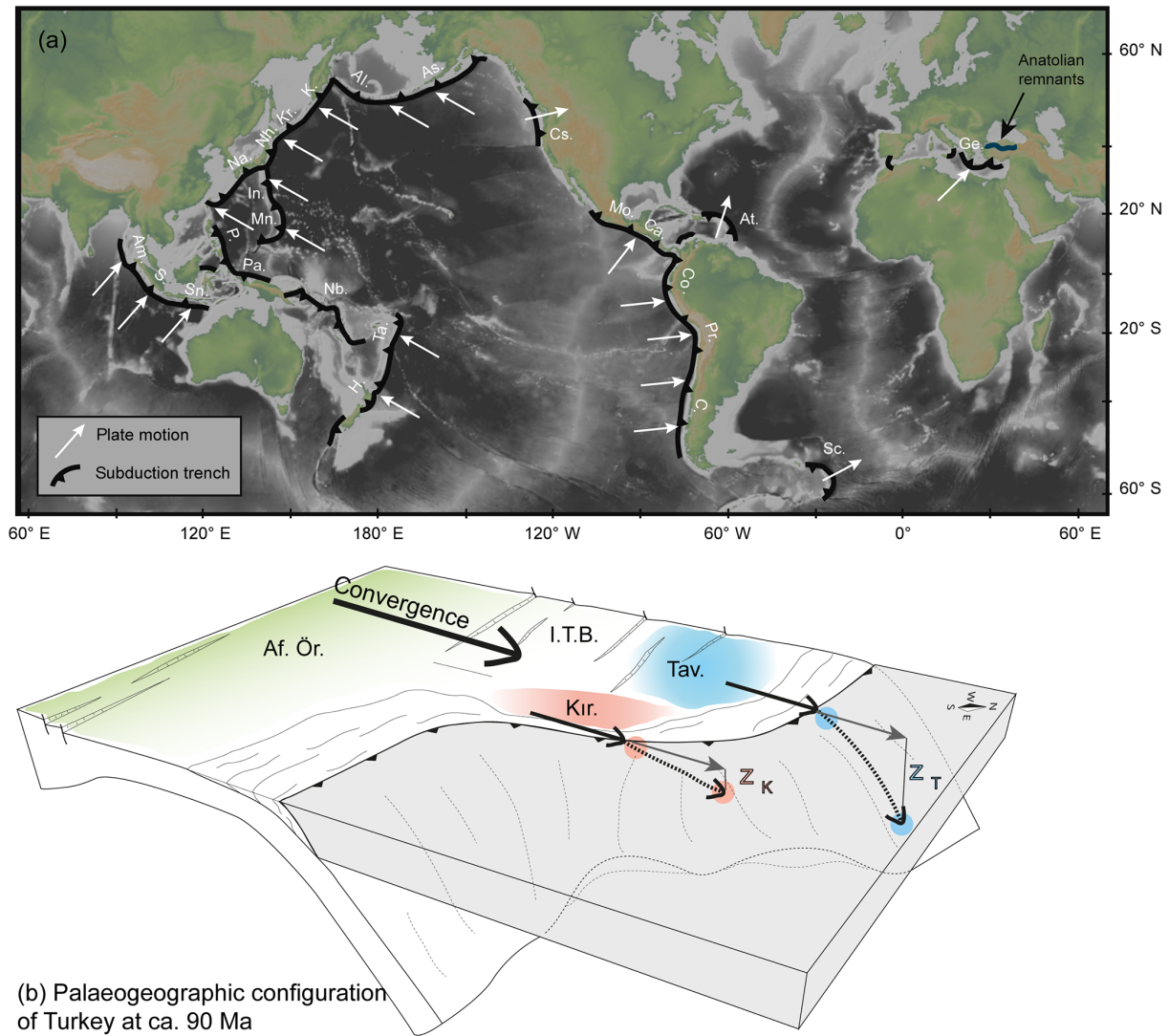
Figure 1. (a) Plate motion at trenches from the NNR-MORVEL model (Argus et al., 2011). Base layer obtained with GeoMapApp ( http://www.geomapp.org , last access: 7 June 2018) with topography and bathymetry from Ryan et al. (2009). Abbreviations as follows: Am., Andaman; As., Alaska; Al., Aleutians; At., Antilles; Ca., Central America; C., Chile; Co. Colombia; Cs., Cascadia; Ge., Greece; H., Hikurangi; In., Izu-Bonin; Nh., Japan; K., Kamchatka; Kr., Kurile; Mn., Marianas; Mo., Mexico; Nb., New Britain; Pa., Palau; Pr., Peru; P., Philippine; S. Sumatra; Sc. Scotia; Sn., Sunda; Ta., Tonga. (b) Possible paleogeographic configuration at ca. 90 Ma for central Turkey based on the reconstruction of van Hinsbergen et al. (2016). Abbreviations correspond to the following units: Af.Ör., Afyon–Ören zone; I.T.B. Inner Tauride Basin; Kir., Kırşehir block; Tav., Tavşanlı zone. Z_K and Z_T refer to the maximum burial of the Kırşehir and Tavşanlı units as discussed in the text.
