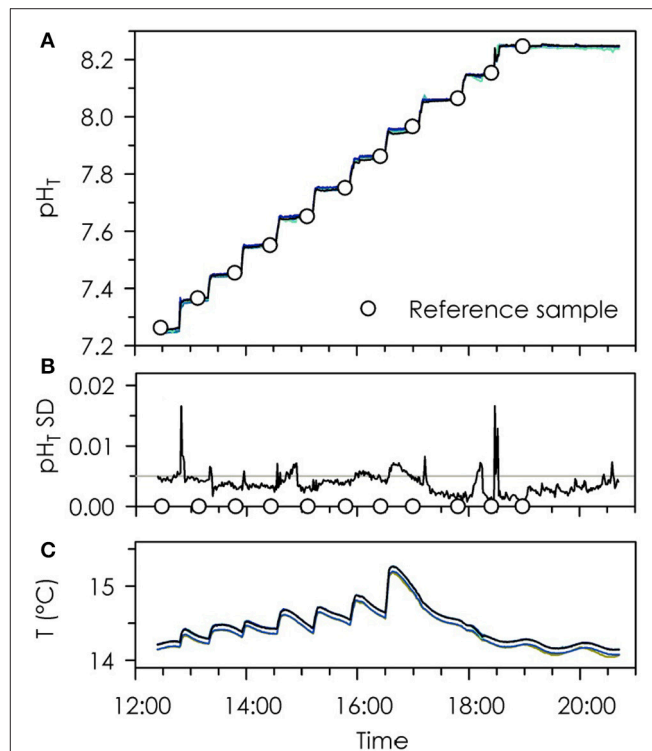
FIGURE 2 | Time-series of pH T ( A ), pH T standard deviation ( B ), and temperature ( C ) of eight Durafet pH electrodes during step-wise increases in seawater pH (lines in A , C are superimposed). Circles represent reference pH samples using the spectrophotometric method with m -cresol purple ( A ) and sample time points ( B ). Reference line in ( B ) indicates a standard deviation of 0.005.
