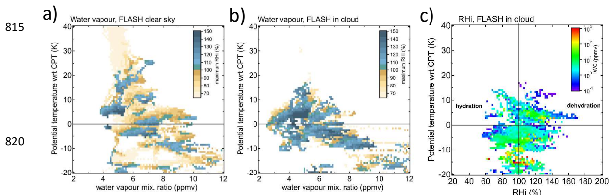
Figure 3. (a) and (b) Binned distribution of maximum RH_i (computed from FLASH and TDC measurements) as a function of FLASH water vapour and potential temperature relative to the local CPT level for (a) clear sky conditions and (b) cloud occurrence detected by MAS (see Sect. 2.1.2). (c) Binned distribution of ice water content (IWC) exceeding 0.1 ppmv from NIXE-CAPS instrument inside clouds detected by MAS as a function of relative humidity over ice ( RH_i ) and potential temperature relative to the local CPT level. The presence of ice crystals in subsaturated air ( RH_i < 100\% ) above the cold point tropopause potentially leads to permanent hydration of the CLS, whereas in supersaturated air the ice crystals are expected to sediment out of the CLS, thereby leading to its dehydration.
