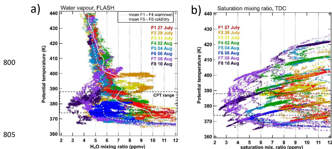
Figure 2. (a) Water vapour mixing ratio profiles taken by FLASH hygrometer. The flight dates are shown in the legend. The dashed rectangle marks the CPT vertical range. The white solid and dashed lines depict the mean water vapour profile for the warm/wet and cold/dry periods respectively (see Fig. 1c, d). (b) Saturation mixing ratio profiles computed from TDC measurements of temperature and pressure. The horizontal dashed lines in both panels mark the vertical range of CPT level encountered during the campaign. Note the strong variability of water vapour at the CPT level and accumulation of sharp enhancements in the lower stratosphere.
