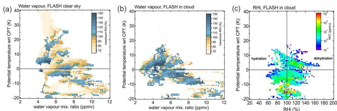
Figure 3. (a, b) Binned distribution of maximum RH i (computed from FLASH and TDC measurements) as a function of FLASH water vapour and potential temperature relative to the local CPT level (bin size 0.1 ppmv by 1 K) for (a) clear-sky conditions and (b) cloud occurrence detected by MAS (see Sect. 2.1.2). (c) Binned distribution of ice water content (IWC) exceeding 0.1 ppmv from NIXE-CAPS instrument inside clouds detected by MAS as a function of relative humidity over ice (RH i ) and potential temperature relative to the local CPT level. The presence of ice crystals in subsaturated air (RH i < 100 %) above the cold point tropopause potentially leads to permanent hydration of the CLS, whereas in supersaturated air the ice crystals are expected to sediment out of the CLS, thereby leading to its dehydration.
