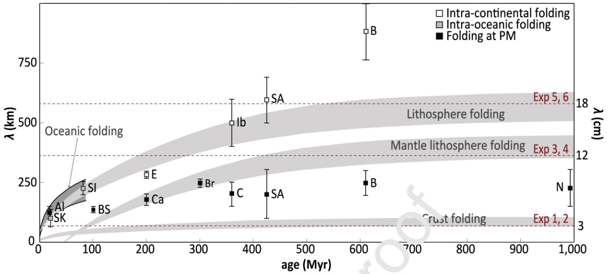
Wavelength of lithosphere folding \lambda vs thermo-tectonic of the lithosphere
