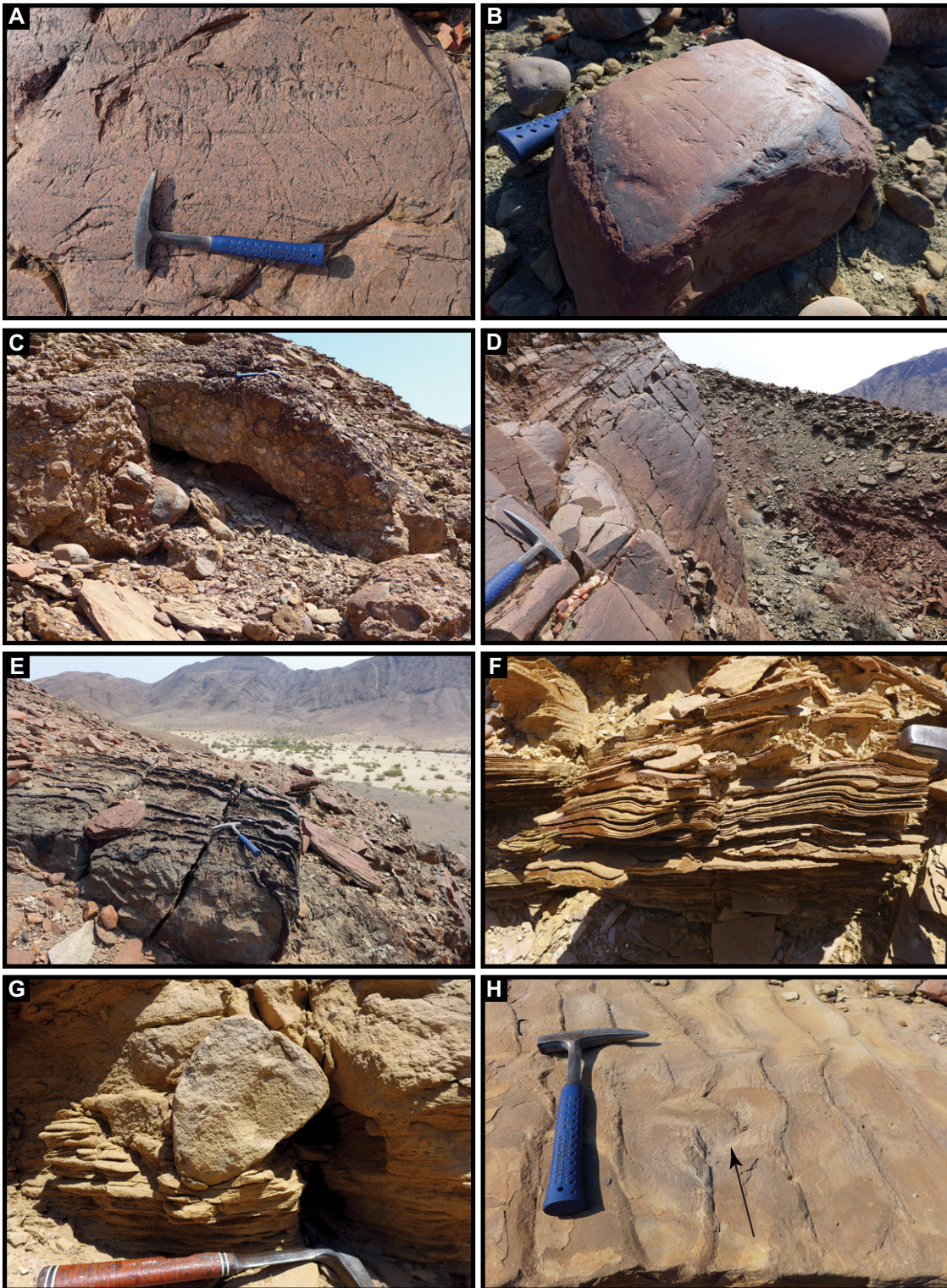
Figure 2. Facies. (A) Striae and crescentic gouges superimposed on roches moutonnées; 18°11'00''S, 12°45'40''E, vertical view. (B) Striated boulder bed covering roches moutonnées; 18°10'46''S, 12°45'45''E, vertical view. (C) Discontinuous and deformed ridge of poorly sorted conglomerate; 18°30'00''S, 12°49'10''E, view toward west. Note hammer near top for scale. (D) Striated vertical wall against which Karoo Supergroup strata abut in background; 18°47'56''S, 13°01'49''E, view toward northwest. (E) Marginal moraine plastered on valley wall, encompassing large erratic boulder; 18°47'53''S, 13°01'45''E, view toward northwest. (F) Rhythmites and sand-mud couplets; 18°29'59''S, 12°49'05''E, view toward south. (G) Lonestone encompassed within sand-sized, rippled sediments; 18°29'59''S, 12°49'05''E, view toward south. (H) Intertidal depositional environment (breached wave ripples) reworking underlying ice-contact fan; 18°29'59''S, 12°49'05''E, view toward south.
