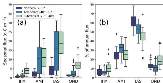
Figure 9. (a) Quarterly contribution to total annual CH 4 flux (in \text{g C m}^{-2} ) and (b) percentage of annual CH 4 flux. Sites were divided into northern (> 60° N), temperate (40–60° N), and subtropical (20–40° N). Quarters with continuous data gaps exceeding 30 d were excluded. We used the following quarterly periods: January–February–March (JFM), April–May–June (AMJ), July–August–September (JAS), and October–November–December (OND). Tropical sites are discussed separately in Sect. 3.3.3 because of their unique seasonality and low number of sites.
