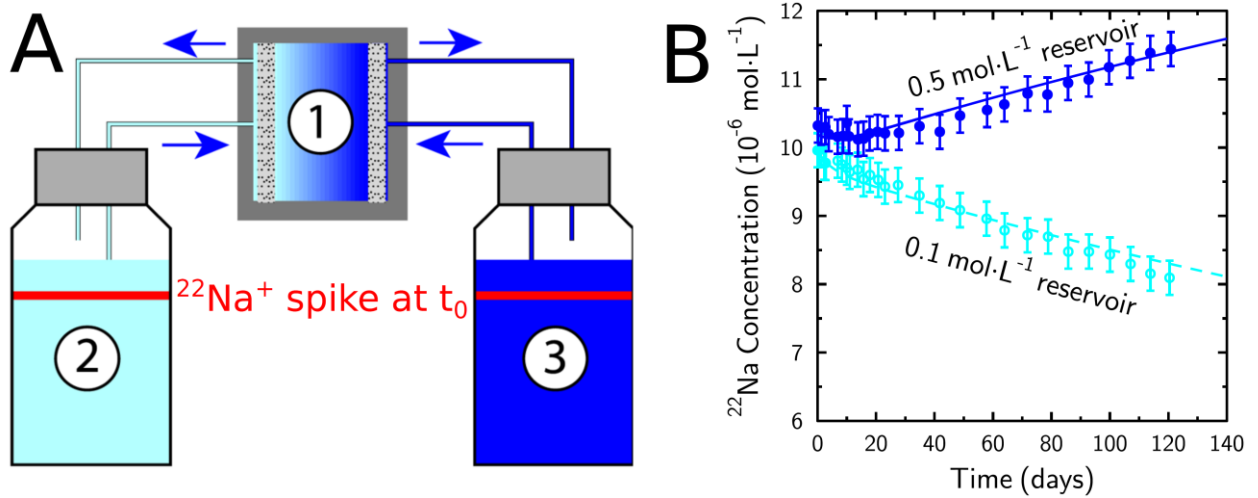
Figure 8. ^{22}Na^+ “Up-hill” diffusion experiment of Glaus et al. (2013). A: experimental setup. The clay sample (1) is in contact with a low salinity reservoir (2) and high salinity reservoir (3) by liquid lines. Blue colors represent the concentration of the background electrolyte; the red bars indicate that the experiment started with equal initial concentrations of the ^{22}Na^+ tracer in the two reservoirs. B: Experimental (symbols) and modeling (lines) results obtained with CrunchClay for the experiment carried out with a \sim 5 mm thick clay plug and reservoir volumes of \sim 250 mL (modified after Glaus et al., 2013 and Tournassat and Steefel, 2015).
