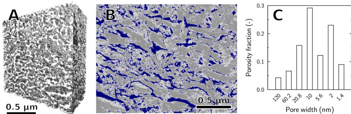
Figure 2. A: 3-D visualization of the microstructure of an illite sample compacted at 1.7 \text{ kg} \cdot \text{dm}^{-3} (backscattered electrons focused ion beam nanotomography stack images 350 \times 350 \times 180 voxels with voxel resolution size of 5 \times 5 \times 5 \text{ nm}^3 ); B: Segmented image of a TEM micrograph of the same illite sample. The blue color represents pores and light and dark gray are pore/solid mixtures and solids, respectively. C: Pore-width distribution obtained from a combination of bulk and microscopic characterization techniques. Figure modified from Gaboreau et al. (2016) and Tournassat et al. (2016b).
