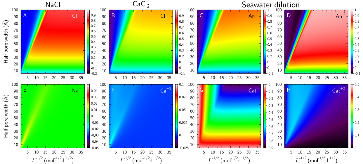
Figure 7. Difference of average diffuse layer concentration values computed with the Poisson-Boltzmann ( C_{PB} ) equation and the Dual continuum model ( C_{Dual} ) model described in Fig. 6 and Eqs. (23) and (24). The difference, given by the color scale, is computed with the equation (C_{PB} - C_{Dual})/C_{PB} as a function of the inverse of the square root of ionic strength ( I^{-1/2} on x-axis) and as a function of the half pore width (y-axis). The equivalence between the two models corresponds to (C_{PB} - C_{Dual})/C_{PB} = 0 . Same caption as in Fig. 5 otherwise.
