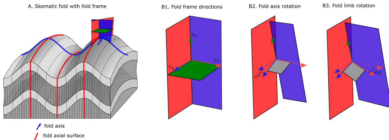
Figure 5. Schematic diagram of a fold adapted from Laurent et al. (2016) showing (a) fold frame, (b1) fold frame direction vectors, (b2) fold axis defined by fold axis rotation angle, (b3) folded foliation defined by fold limb rotation around fold axis.
