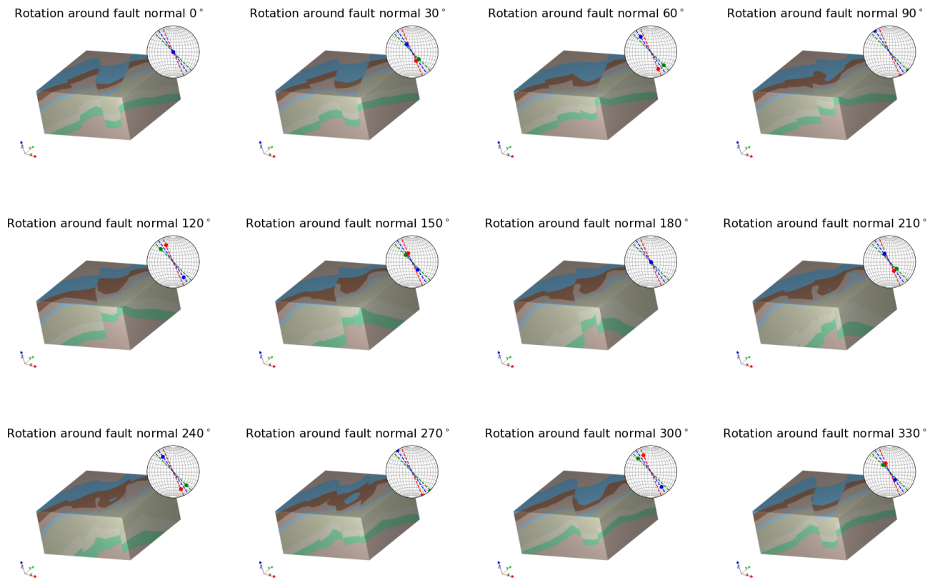
Figure 14. The 12 model iterations where initial fault slip vector has been rotated around the normal to the fault surface. Stereonets show the resulting fault slip vectors (poles) and the fault plane (great circles).
