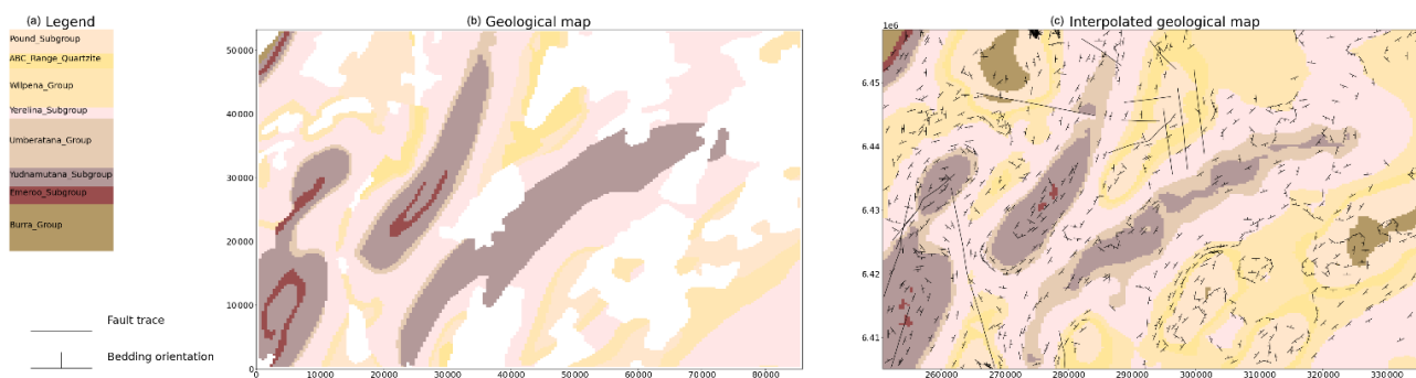
Figure 12. (a) Stratigraphic column for model area showing relative thickness. (b) Geological map showing bedding and faults. (c) Geological model shown on map surface.
