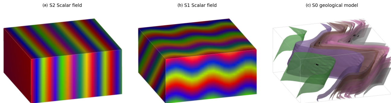
Figure 11. Scalar fields: (a) S2, (b) S1 and (c) bedding.
