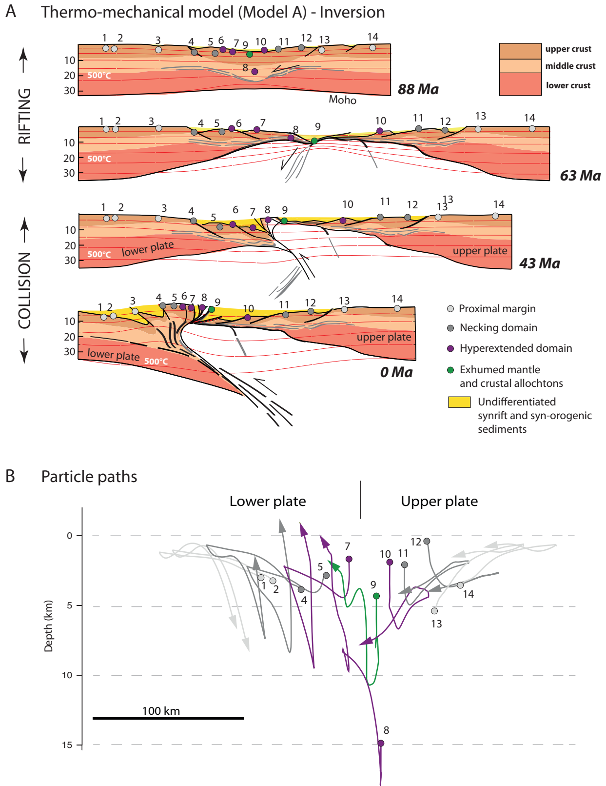
Fig. 1. (A) Crustal temperature evolution of an inverted rift system based on thermo-mechanical modelling by Jourdon et al. (2019) (Model A). The location of the fourteen upper crustal basement particles selected for forward modelling of low-temperature thermochronology data is indicated. (B) Spatial and temporal evolution of the fourteen particles studied with regards to their final position within the orogenic system, indicating periods of burial/exhumation as well as maximum depths reached throughout entire particles' rifting-to-collision history. Path colours correspond to the domain colour scheme defined in (A). Each particle (or path) number is labelled according to the position of the particle in the final orogenic prism from the lower, downgoing plate to the upper plate in Model A.
