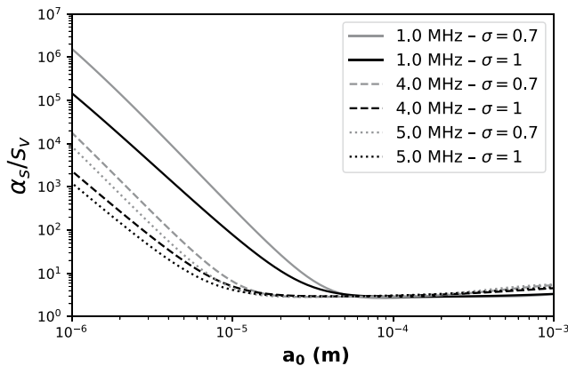
Figure 11. theoretical ratio \alpha_s/s_v as a function of the median radius a_0 of the lognormal volume Particle Size Distribution for \sigma = 0.7 and \sigma = 1.0 at 1.0, 4.0, and 5.0 MHz.
