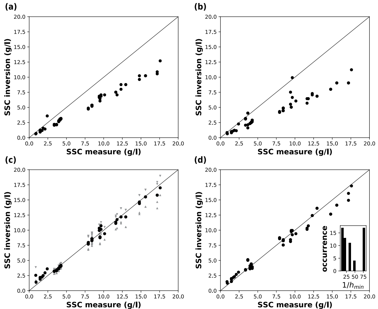
Figure 12. Multifrequency backscatter and attenuation inversion (Method 4): (a) case M4.1 (cf. Table 1), (Urlick, 1948) spherical model, lognormal Particle Size Distribution [PSD]; (b) case M4.2, spherical model, bimodal PSD; (c) case M4.3 (Richards et al., 2003), oblate spheroid model, lognormal PSD, minimum particle aspect ratio ( h_{\min} ) set to 1/40 (black circles). Downward and upward gray triangles show inverse suspended sediment concentration (SSC) range for h of 1/80 and 1/20 respectively; (d) case M4.4, inverting h_{\min} in addition to PSD parameters and SSC, the obtained values for h_{\min} are represented on a histogram in the bottom right corner. Solid lines show perfect agreement.
