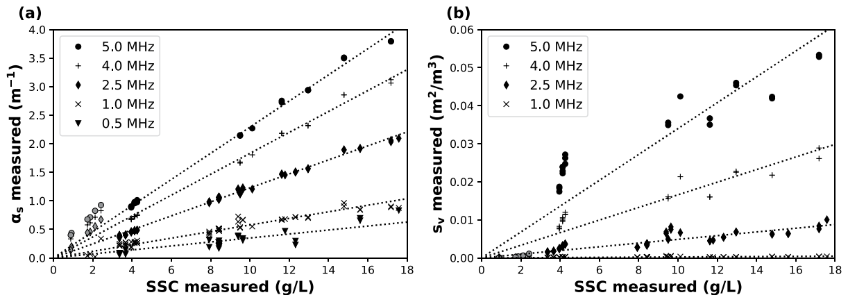
Figure 5. Measured suspended sediment concentration versus (a) measured sediment attenuation ( \alpha_s ) and (b) range-averaged measured volume backscattering coefficient ( s_v ). Dashed lines are regression lines forced to the origin computed for constant Particle Size Distribution (PSD) data. Gray points indicate that the pumps were turned off in the tank and correspond to different PSD.
