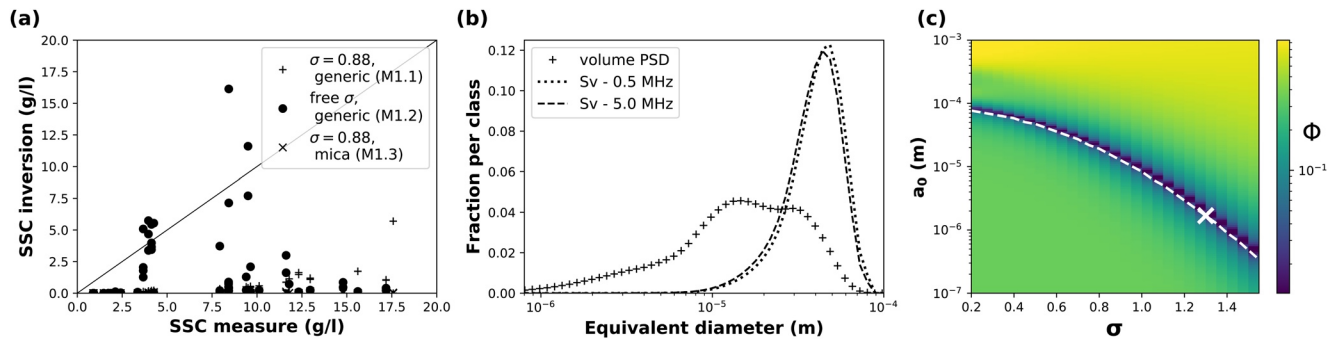
Figure 8. Backscatter multifrequency inversion outputs (Method 1): (a) inverse suspended sediment concentration (SSC) versus measured SSC, in the cases of Particle Size Distribution (PSD) width ( \sigma ) fixed prior to the inversion (case M1.1 of Table 1), \sigma left free in the inversion (case M1.2), using the mica-specific model instead of the generic model (case M1.3). A solid line is perfect agreement line; (b) mean volume PSD measured by laser diffraction (crosses) and contribution to s_v per size class at 0.5 and 5.0 MHz (dashed lines); (c) example of \Phi inversion objective function (Equation 6) values in the parameter space ( a_0 , \sigma ), the white dashed line shows the local minimum valley, the cross indicates the location of the absolute minimum of \Phi that is used to retrieve the inverse parameters (SSC, a_0 , and \sigma in this case).
