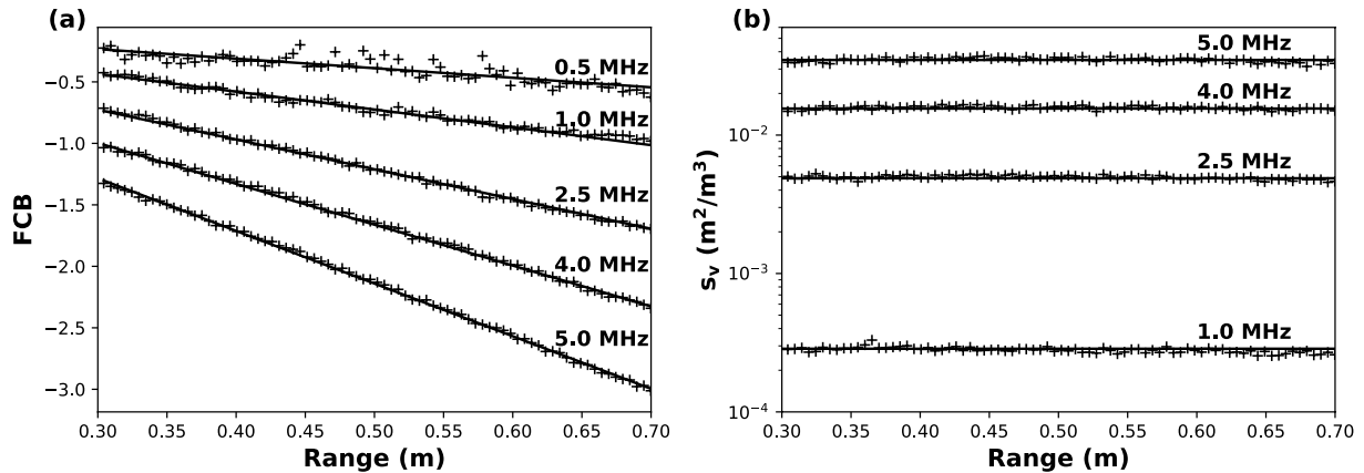
Figure 4. Example of profiles (crosses) with linear fit recorded in the tank for M \approx 9.5 g/l: (a) fluid corrected backscatter (FCB); (b) volume backscattering coefficient ( s_v ). The intercepts of the FCB profiles were set to 0 for r = 0 to make the slopes comparison easier.
