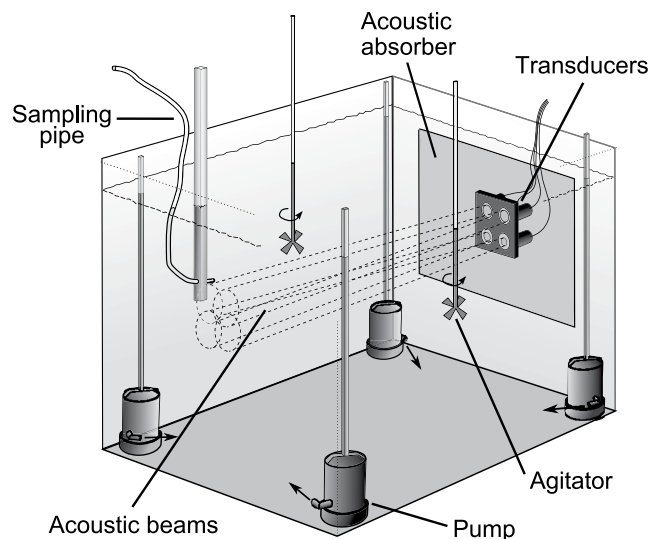
Figure 2. Experimental tank ( 1 \times 1 \times 1 m) used in this study. A second tile of acoustic absorber was fixed on the wall facing the transducers (not shown here).
