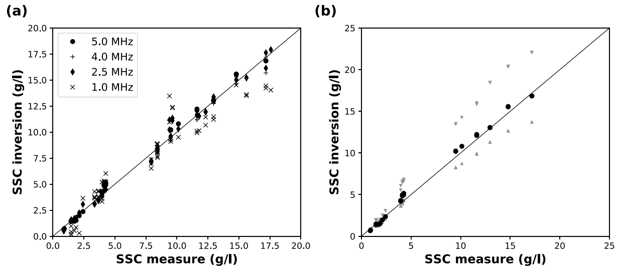
Figure 10. Single-frequency backscatter and attenuation inversion outputs (Method 3): (a) for the various sonar frequencies, with Particle Size Distribution width ( \sigma ) set to 0.88; (b) at 5.0 MHz, inverse suspended sediment concentration for \sigma = 0.88 (circles), \sigma = 0.7 (downward triangles) and \sigma = 1.0 (upward triangles). Solid lines show perfect agreement.
