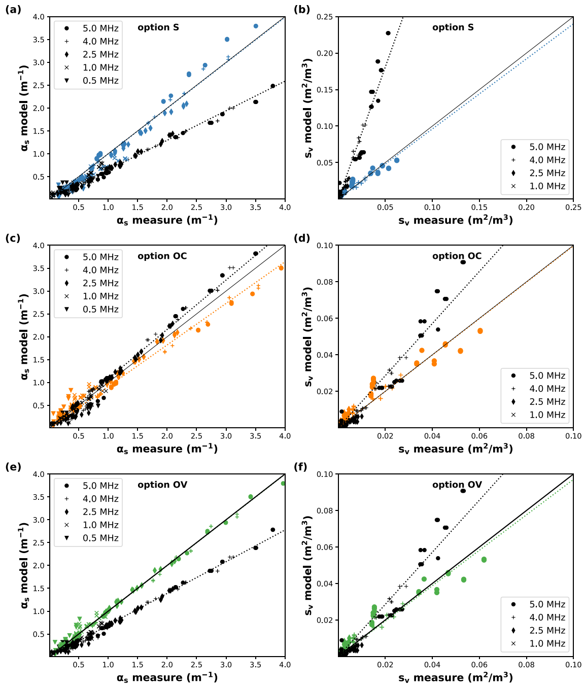
Figure 6. Acoustic model outputs versus measurements for all available sonar frequencies: in black, direct modeling using the Particle Size Distribution (PSD) data measured by laser diffraction; in blue, orange and green, direct modeling using the optimal PSD obtained from the sensitivity test—optimal PSDs are shown in Figure 7 with colors matching the present figure. (a) and (b) Sediment attenuation ( \alpha_s ) and volume backscattering ( s_v ) using option S; (c) and (d) option OC; (e) and (f) option OV. Model equations, used parameters, linear regression slopes and goodness of fit R^2 for the three options S, OC, and OV are summarized in Table 3.
