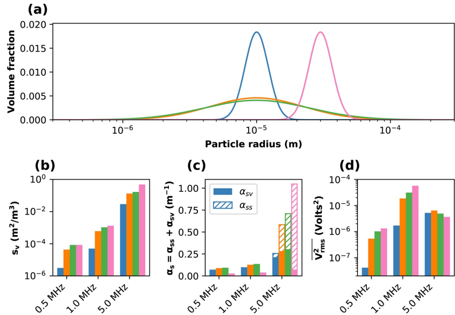
Figure 1. Examples of acoustic model results for spherical particles, with a suspended sediment concentration of 4 g/l, for three frequencies. (a) Synthetic Particle Size Distributions (PSDs) used for the computation. (b) Backscatter ( s_v ) for the corresponding PSD, the color of the bar corresponds to the PSD represented with the same color. (c) Sediment attenuation ( \alpha_s ): contributions of scatter ( \alpha_{ss} ) and viscous ( \alpha_{sv} ) effects. (d) Resulting synthetic signal V_{rms}^2 at r = 1 m.
