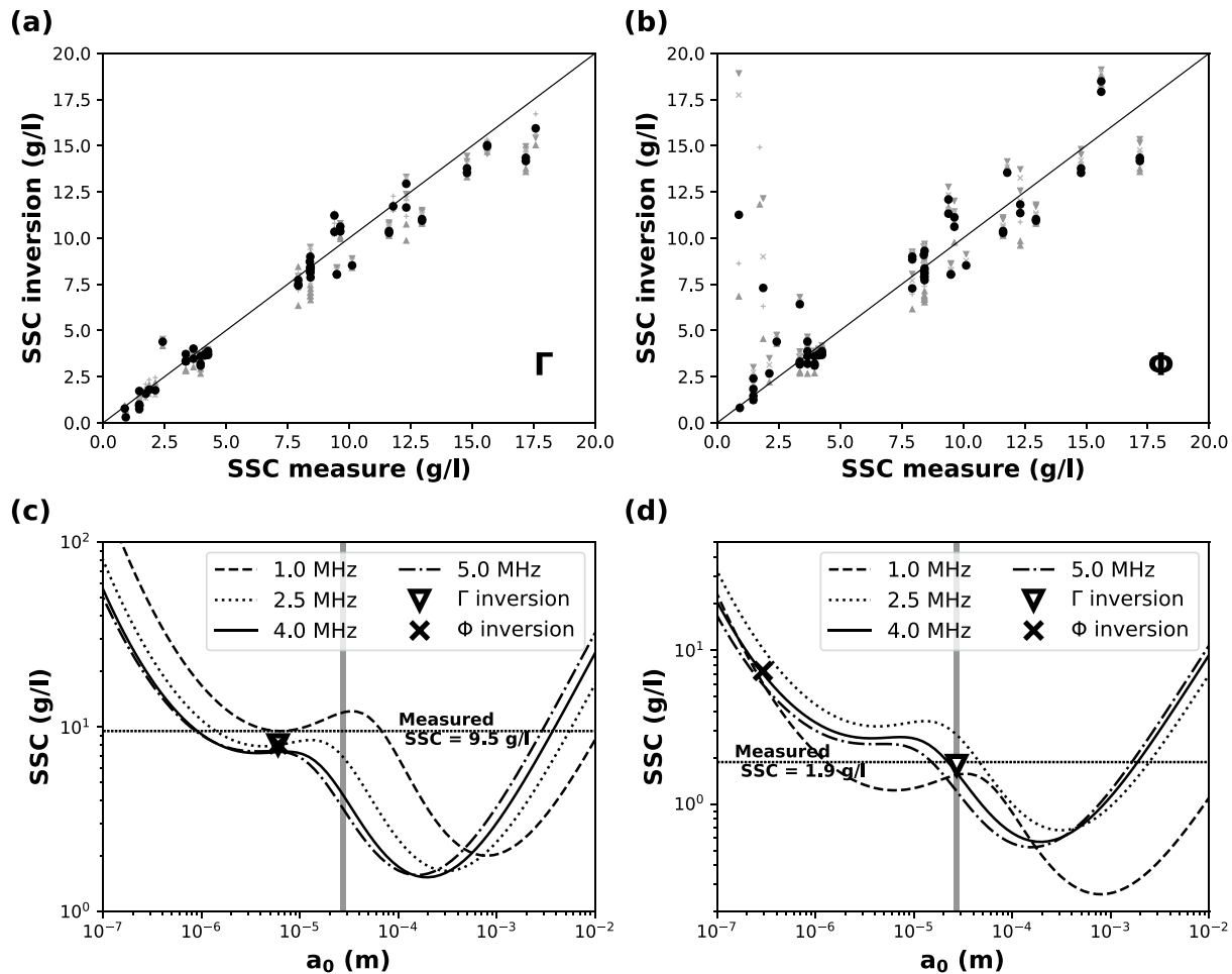
Figure 9. Multifrequency attenuation inversion outputs (Method 2), case M2.3 (cf. Table 1). (a) and (b) Inverse suspended sediment concentration (SSC) versus measured SSC using the \Gamma objective function (a); using the \Phi objective function (b). Black circles show inverse SSC for \sigma = 0.88 and h = 1/40 . Downward and upward gray triangles show inverse SSC for h = 1/80 and h = 1/20 , respectively. Crosses (+) and (x) show inverse SSC for \sigma = 0.7 and \sigma = 1.1 , respectively. The solid line shows perfect agreement. (b) and (c) Examples of SSC modeled from measured acoustic attenuation at various frequencies in case M2.3 (cf. Table 1) versus the median radius ( a_0 ) of the volume lognormal Particle Size Distribution (assumed lognormal) for two different concentrations: (b) SSC = 9.5 g/l; (c) SSC = 1.9 g/l. Horizontal lines show the measured SSC, vertical gray lines show the upper limit set to a_0 in the inversion process, crosses, and triangles show inversion outputs using \Phi and \Gamma objective functions, respectively.
