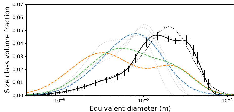
Figure 7. Volume particle size distribution: average of all the laser diffraction measurements (solid black line with error bars including all measurements), excluding the last samples with the pumps off (Particle Size Distribution [PSD] shown as light gray dotted lines); 2-mode Gaussian mixture model fit to the mean PSD (dotted black line); PSD leading to the best agreement between model outputs ( \alpha_s and s_v ) and the measurements, using the spherical model (option S, dashed blue line) or oblate spheroid model for viscous attenuation, with constant h (option OC, dashed orange line) or varying h (option OV, dashed green line). Model equations and used parameters for these options are summarized in Table 3.
