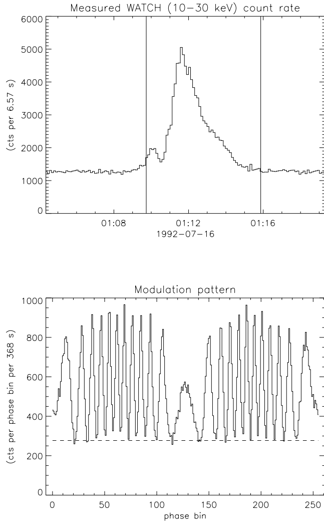
Fig. 1. The time profile of a solar event (top) with corresponding modulation pattern (bottom). The background estimated in the countrate time profile before and after the burst is indicated as a dotted line in the modulation pattern.
