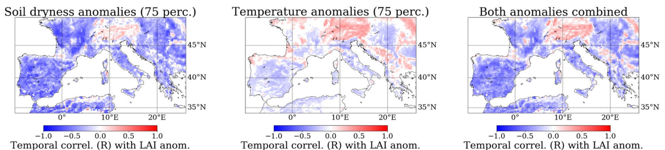
Fig. 8 Spatial distribution of temporal correlation (R) during summers (2003–2016) between MODIS LAI anomalies and PLA_{SD} (left), PLA_{T2m} (middle) and combined PLA_{SD,T} (right). White cells correspond to non-significant correlation coefficients (Spearman
