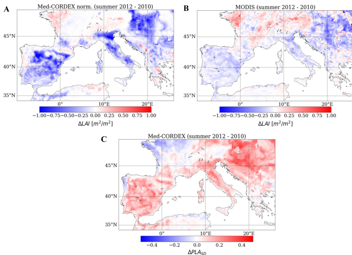
Fig. 7 Spatial distribution of mean \Delta\text{LAI} between the summer of 2012 and 2010 with the Med-CORDEX simulation normalized (A) and MODIS observations (B). Spatial distribution of the mean \Delta\text{PLA}_{SD} with the Med-CORDEX simulation (C)
