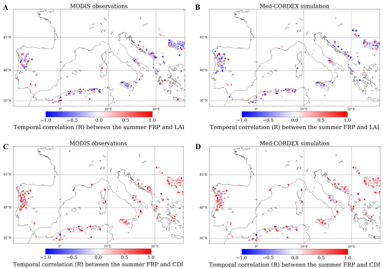
Fig. 11 Spatial distribution of temporal correlation ( R ) between summer Fire Radiative Power (FRP) and Leaf Area Index (LAI) from MODIS ( A ) and from Med-CORDEX ( B ) for areas of high fire activity (pixels with at least 1 \text{ km}^2 of burned area for minimum 3 summers over 2003–2016). Same criteria of correlation are applied
