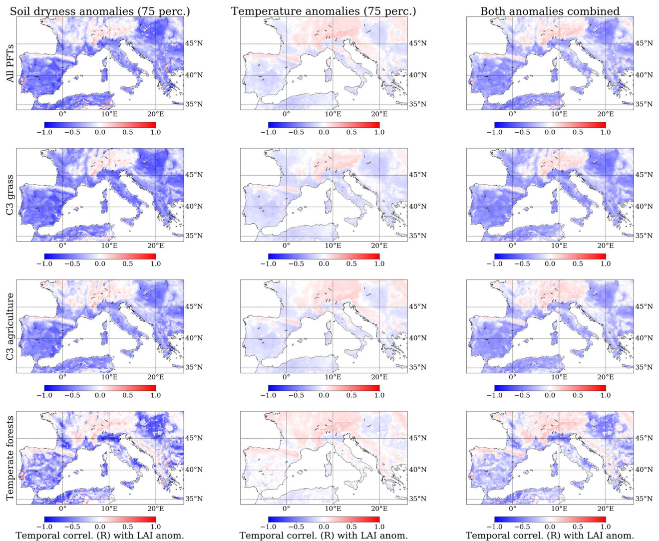
Fig. 9 Spatial distribution of temporal correlation ( R ) during summers (1979–2016 period) between Med-CORDEX LAI anomalies and PLA_{SD} (left), PLA_{T2m} (middle) and combined PLA_{SD,T} (right).
