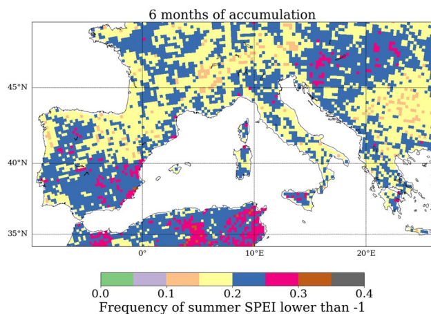
Fig. 5 Spatial distribution of frequency of summer SPEI lower than -1 computed with 6 months of accumulation period. The frequency is expressed over the total number of summer months along the simulation period, namely 114 months
