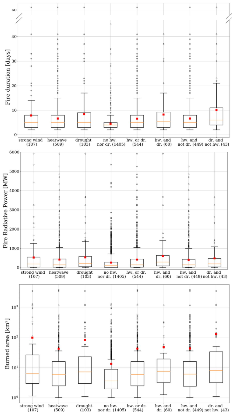
Fig. 10 Summer Burned Area (bottom panel on log scale), Fire Radiative Power (middle panel), and Fire Duration (top panel), observed by the MODIS satellite instrument during isolated and combined extreme events over the Western Mediterranean, represented by individual boxplots. From left to right are the clusters using the PLA method: “windspells”, “heatwaves”, “droughts”, “no heatwave nor drought”, “heatwaves or droughts”, “simultaneous droughts and heatwaves”, “heatwaves without droughts” and “droughts without heatwaves”. Only fire lasting more than 1 day and burning more than 1 km 2 are kept. Fires next to each other, and separated by 2 days, are grouped into the same fire event. The number of fire events is between the parentheses. The red squares are the mean of the distribution and the black circles are the outliers. The box covers the InterQuartile Range (IQR) between Q1 (25th percentile) and Q3 (75th percentile). The lower whisker is limited to a statistical minimum ( Q1 - 1.5 \cdot IQR ) and the upper one to a statistical maximum ( Q3 + 1.5 \cdot IQR )
