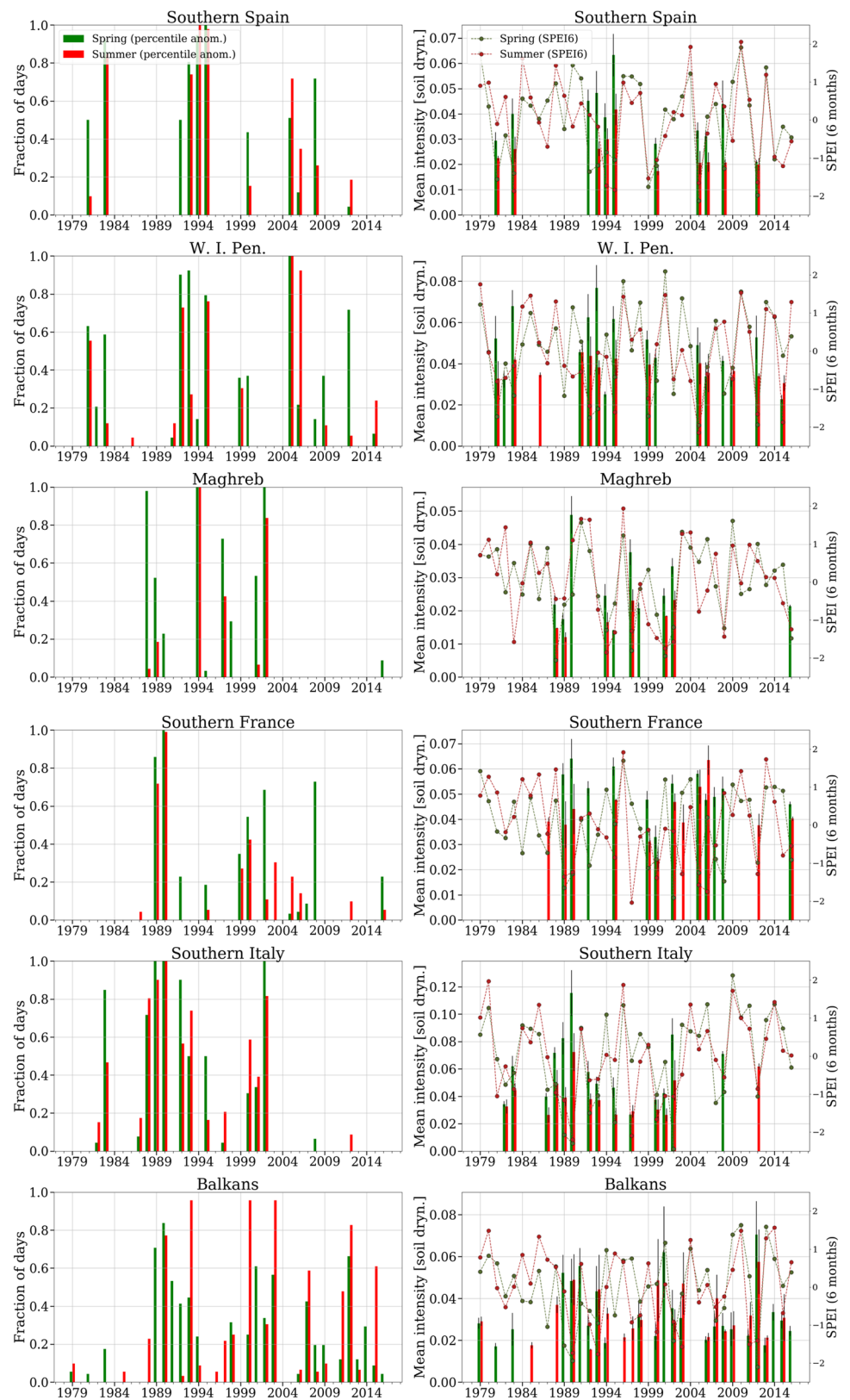
Fig. 6 Temporal variation of spring (MAM) and summer (JJA) agricultural droughts for the sub-regions defined in Fig. 1 using the PLA_{SD} method (on soil dryness). Left column: fraction of days affected. Right column: mean PLA_{SD} and SPEI (intensity)
