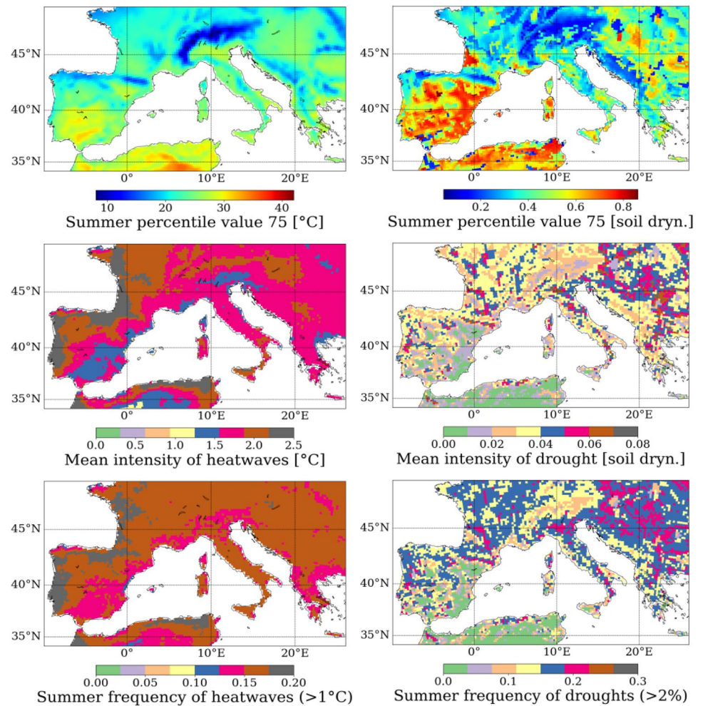
Fig. 4 Heatwaves (left column) and droughts (right column) identified using the Percentile Limit Anomalies (PLA) method. The first row shows the 75th percentile value during summer (JJA average), the second row shows the mean intensity of the extreme events, and the last row shows the frequency (over the total number of summer days) of intense events ( > 1^\circ\text{C} for heatwaves and > 0.02 of soil dryness for droughts)
