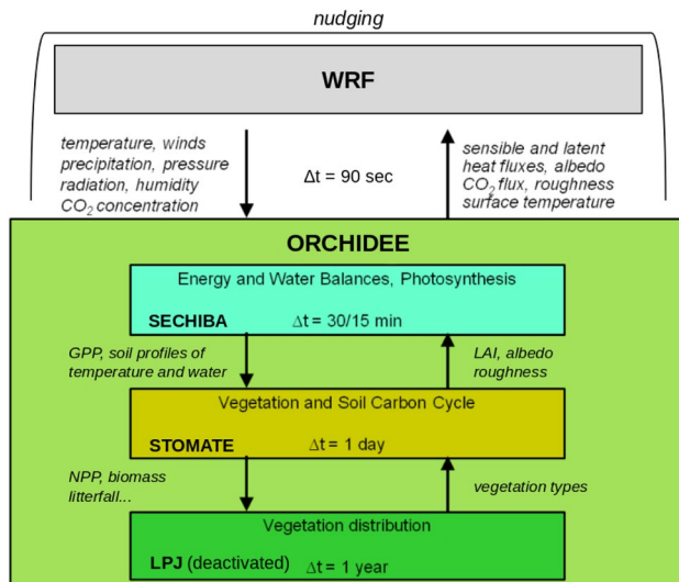
Fig. 2 The RegIPSL coupling flow chart. This figure is inspired by the IPSL online documentation ( https://orchidee.ipsl.fr/ )
